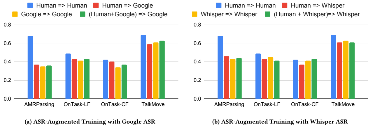
Figure 2: Main Results for ASR-Augmented Training on AMRPARSING, ONTASK (Lesson-Focused, Classroom-Focused) and TALKMOVE. In the legend, "A=>B" means the model is trained on A, and evaluated on B.
