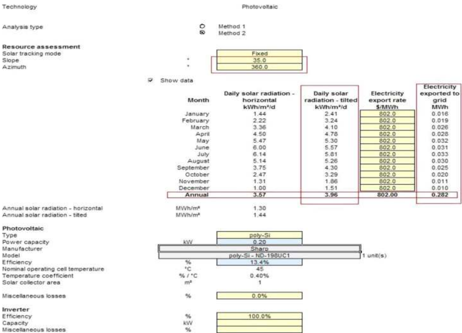
Fig. 4 RETScreen interface
