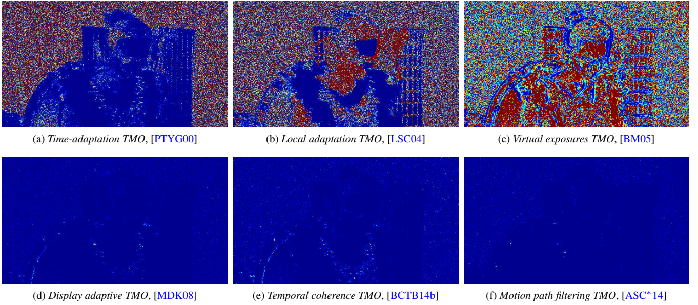
Figure 10: Examples of measured local (per-pixel) temporal coherence, where blue and red corresponds to good and poor coherence, respectively. The examples demonstrate three TMOs that have problems with local temporal coherence (a)-(c), and three that show good coherence (d)-(f). Even though local incoherence is mostly associated with local TMOs (b)-(c), the global operator in (a) also suffers from incoherence due to amplified noise in the darker parts of the image. The frames are taken from measurements using Equation 26 on tone-mappings of the Showgirl HDR video sequence in Figure 19.
