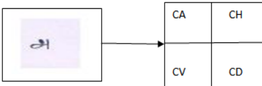
FIG.2 WAVELET DECOMPOSITION
