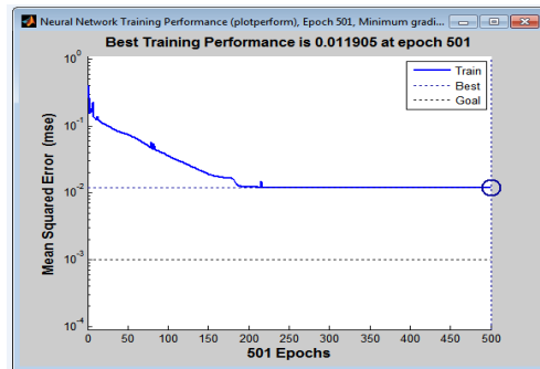
FIG.10 PERFORMANCE PLOT FOR DB1 WAVELET
