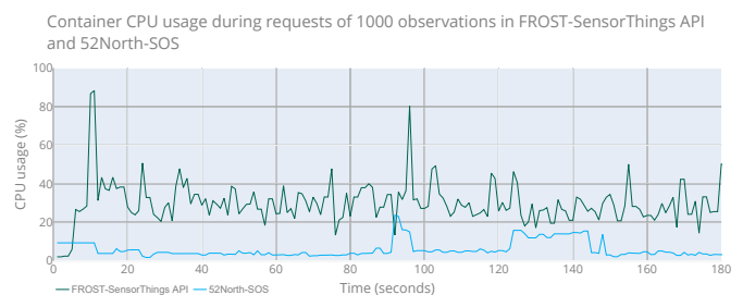
Fig. 7. CPU usage behaviour from FROST-SensorThings API and 52North-SOS during responses of 1000 observations.
