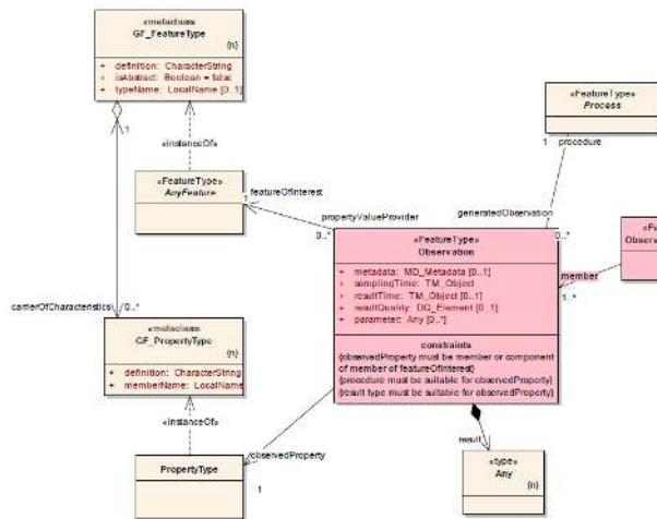
Fig. 1. O&M data model extract [17].
