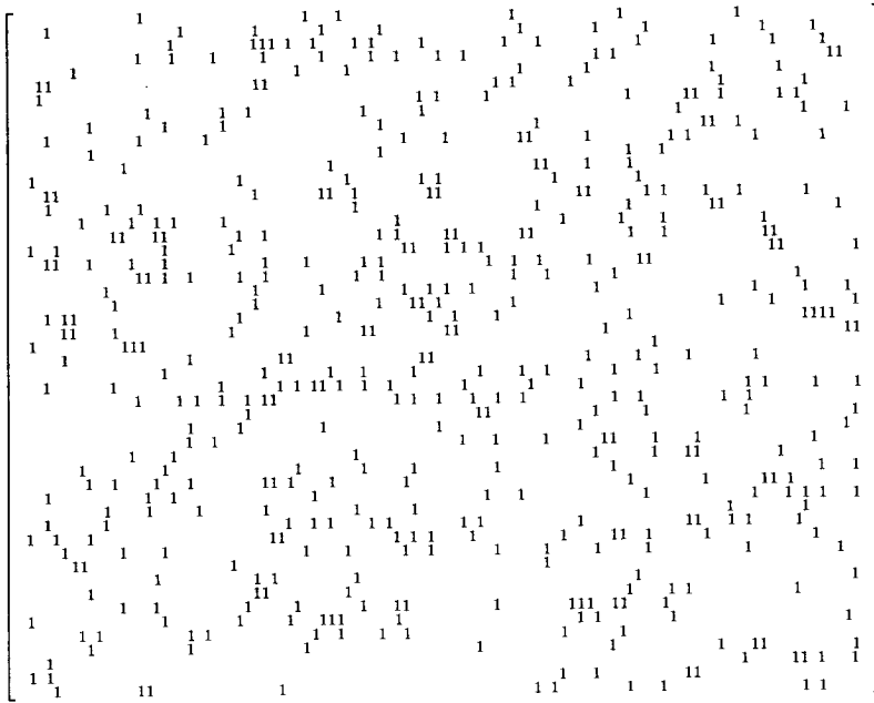
(a) Clumpiness = 1
