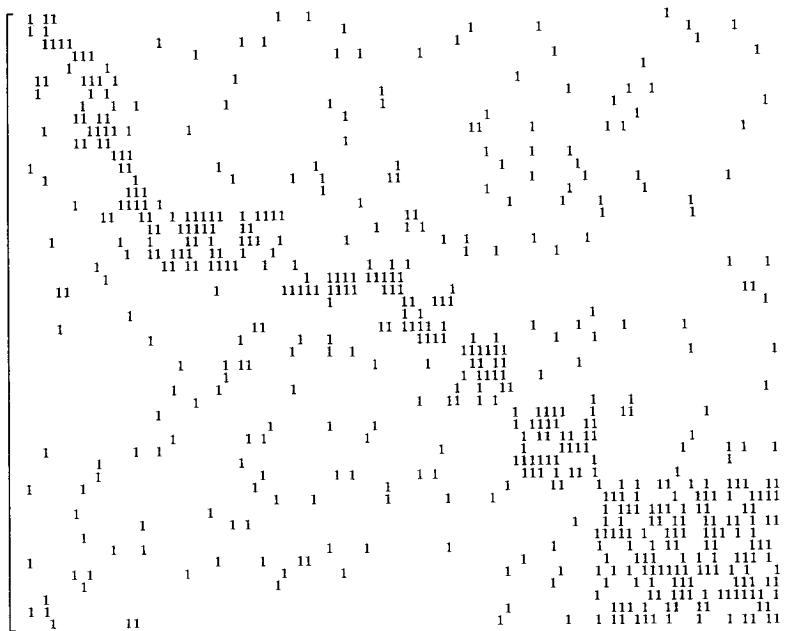
(b) Clumpiness = 2
