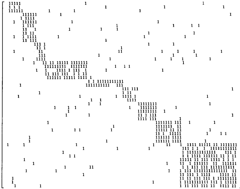
(c) Clumpiness = 4
