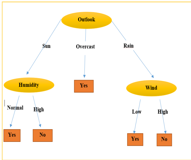
Fig. 3. ID3 Final tree
