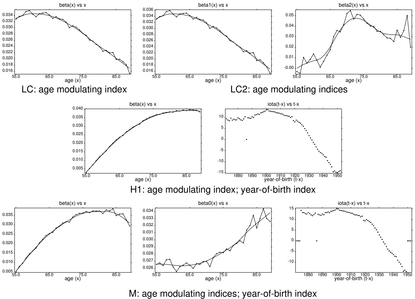
Fig 9. England & Wales 1961-2007 male mortality experience, ages 55-89. Binomial responses, log-odds link, target q(x,t) , predictors LC, LC2, H1, M.
