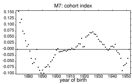
Models M6-M8: year-of-birth indices
