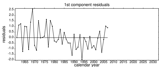
Model LC2: deviance residual plots
