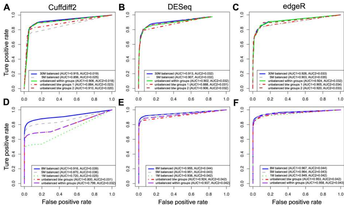
Figure 6. The effects of balanced and unbalanced depths of reads for detecting DEGs based on ROC curve. ROC curves for evaluating the performance of Cuffdiff2, DESeq and edgeR on balanced and on unbalanced depths of reads based on the K_N dataset (A–C) and the LCL3 simulated dataset (D–F). doi:10.1371/journal.pone.0103207.g006
