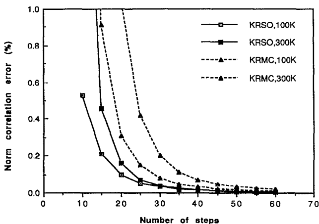
FIG. 7. The correlation error (%) of the norm of the final thermal wave function plotted vs the total number of steps for the kinetic referenced split operator (KRISO) and kinetic referenced modified Cayley (KRMC) methods.
