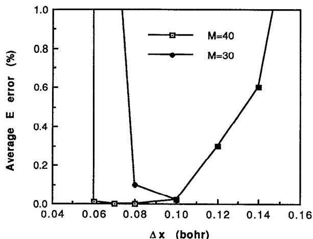
FIG. 5. The average energy error (%) plotted vs the grid spacing \Delta x for the Chebyshev polynomial expansion method for the order of M = 30 and 40 . The time step is 1 fs for the total time of 1 ps, and N is 64 in this case.
