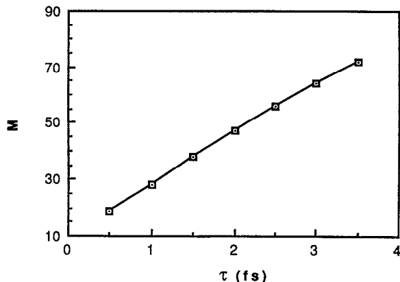
FIG. 6. The minimum order of the Chebyshev polynomial expansion which gives the error of less than 0.1% in error measures in the norm and the energy plotted vs the time step (fs).
