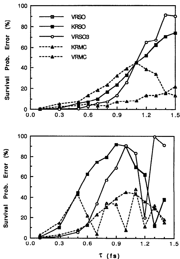
FIG. 2. The survival probability error (%) plotted vs the time step (fs) for the second and third order potential referenced split operator (VRSO and VRSO3, respectively), kinetic referenced split operator (KRSO), and kinetic and potential referenced modified Cayley (KRMC and VRMC, respectively) methods. (a) is for the total time of 1 ps and (b) is for the total time of 5 ps. The grid spacing, \Delta x , is 0.04, and N , the number of x -grid points is 256. The results for VRSO and KRSO are nearly identical.
