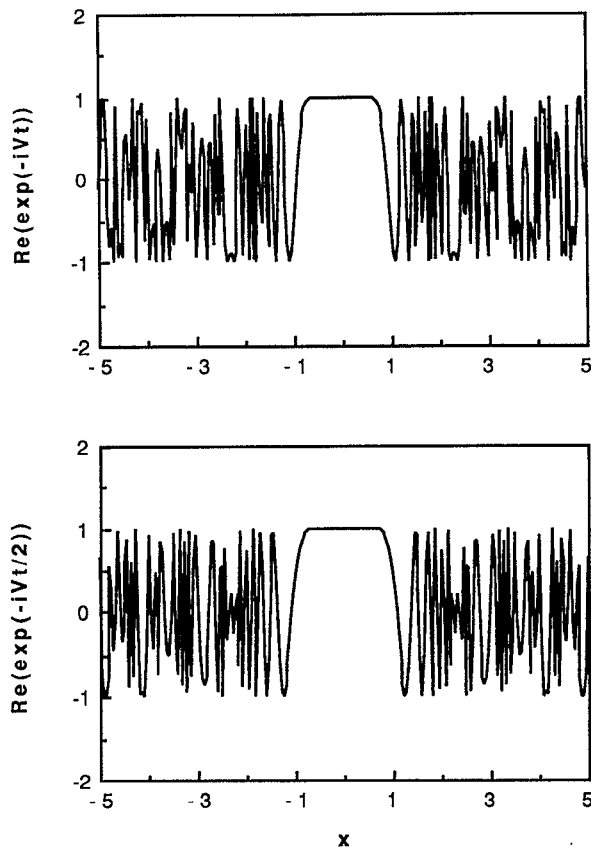
FIG. 4. The real components of the exponential unsplit and split potential operators, \text{Re}[\exp(-iVt)] and \text{Re}[\exp(-iVt/2)] , respectively, are plotted vs the coordinate x in atomic units. The time t is 1 fs.
