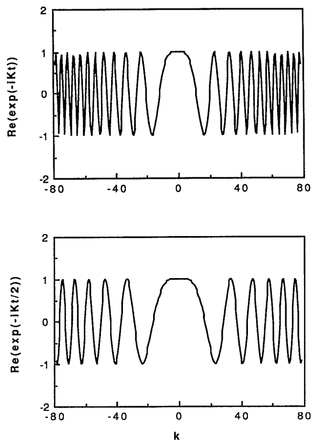
FIG. 3. The real components of the exponential unsplit and split kinetic operators, \text{Re}[\exp(-i\mathbf{K}t)] and \text{Re}[\exp(-i\mathbf{K}t/2)] , respectively, are plotted vs the momentum k in atomic units. The time t is 1 fs.
