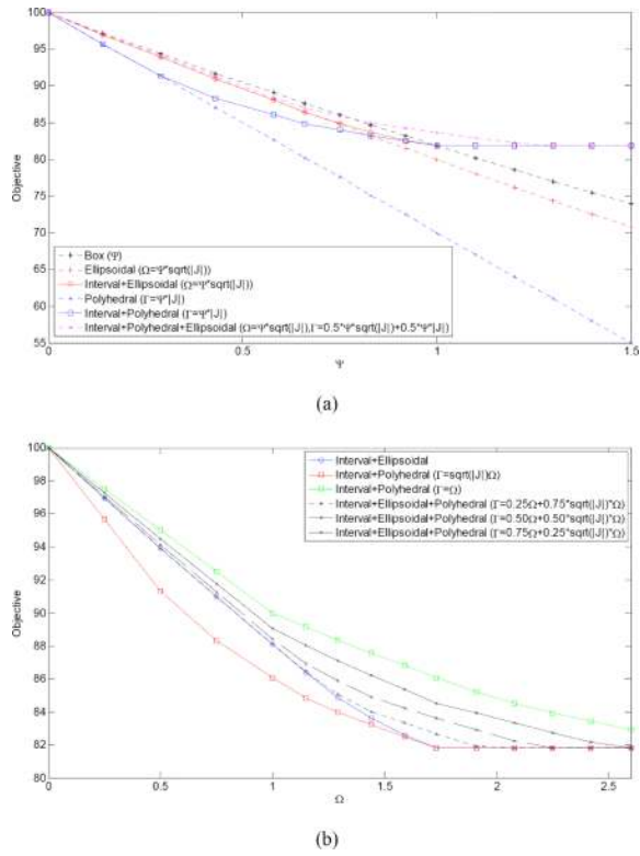
Figure 5.3. Simultaneous LHS and RHS uncertainty for both constraints ( |J_i| = 3 )
