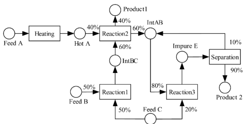
Figure 7.6. State Task Network (STN) representation of the batch chemical process
