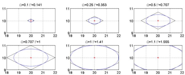
Figure 3.8. Illustration of the relationship between ellipsoidal and polyhedral uncertainty set ( \Gamma=\Omega \sqrt{2} )
