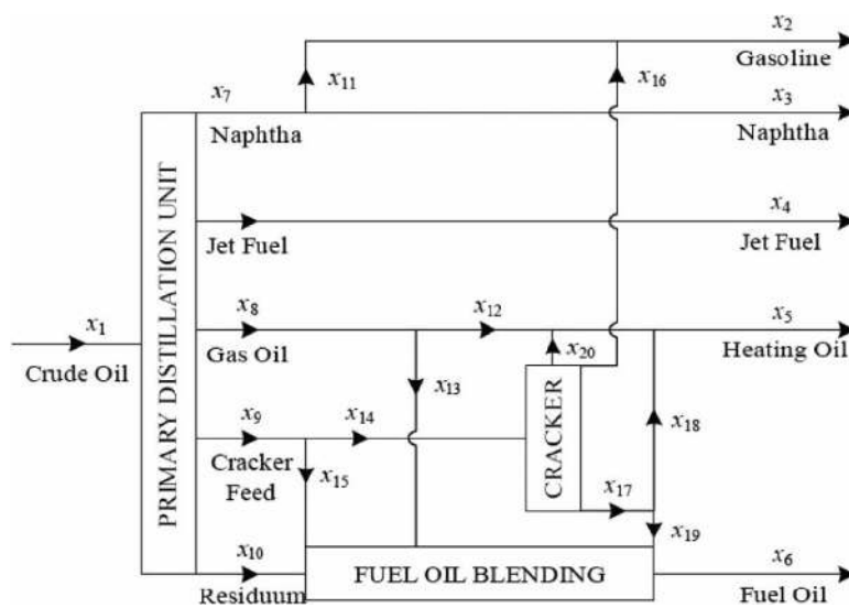
Figure 5.5. Refinery flowchart
