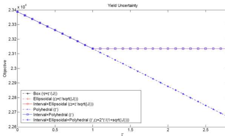
Figure 5.6. Solution for yield uncertainty
