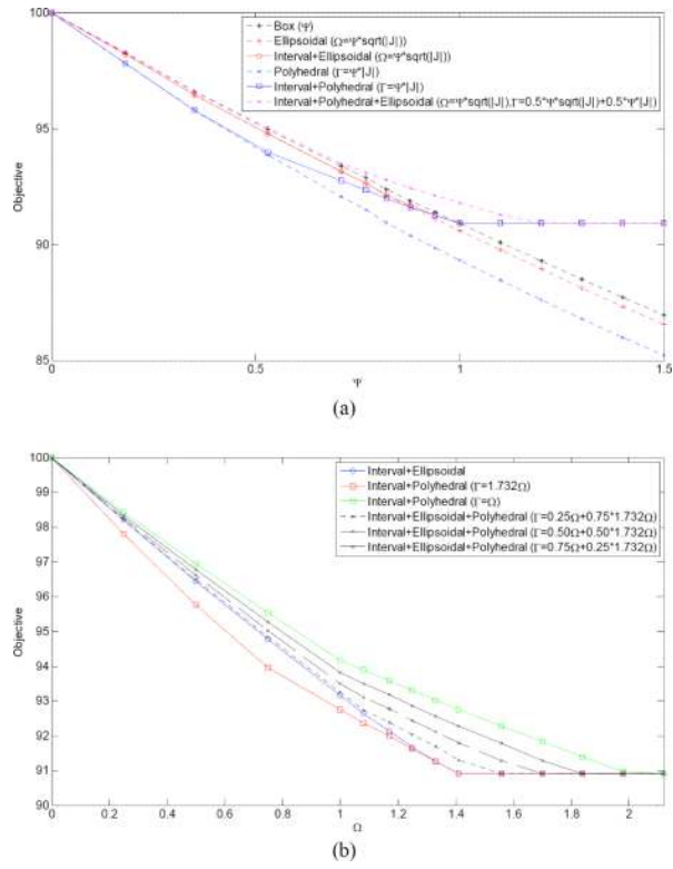
Figure 5.1. Only LHS uncertainty for both constraints ( |J_i| = 2 )
