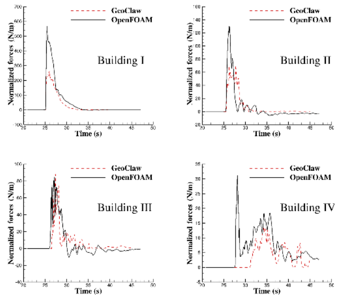
Figure 15. Predicted forces in cross-shore direction on selected buildings (normalized).
