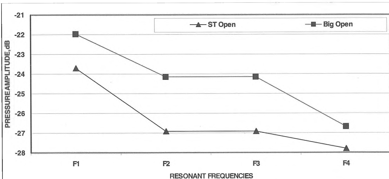
Figure 4. Impedance Measures of the Open Headjoint (Standard and Bigio S/C) for Minima Corresponding to the Headjoint's Resonant Frequencies.
