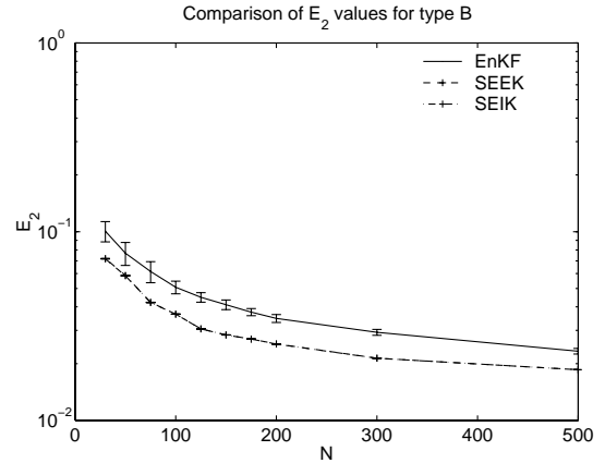
Figure 5. Normalized time integrated estimation errors for the three filter algorithms as a function of the ensemble size N for experiments of type B with excellent initial guess. The lines of the SEEK and SEIK filters lie on top of each other. Error bars describe the spread due to the use of random numbers.
