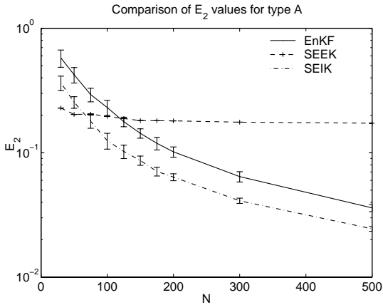
Figure 4. Normalized time integrated estimation errors for the three filter algorithms as a function of the ensemble size N ( N = r + 1 for SEEK and SEIK) for experiments of type A with poor initial guess. Error bars describe the spread due to the use of random numbers.
