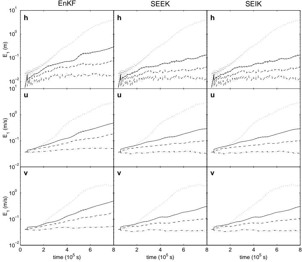
Figure 6. RMS Estimation errors for experiments of type B with excellent initial guess. Shown is the time development of the error of the assimilated state for three ensemble sizes ( N=30 (solid line), 100 (dashed), 500 (dash-dotted)) and for a model simulation without assimilation (dotted line). Each column shows the results for one particular filter algorithm. The three rows show the different model fields. As in case A, filter performance and divergence is a function of ensemble size.
