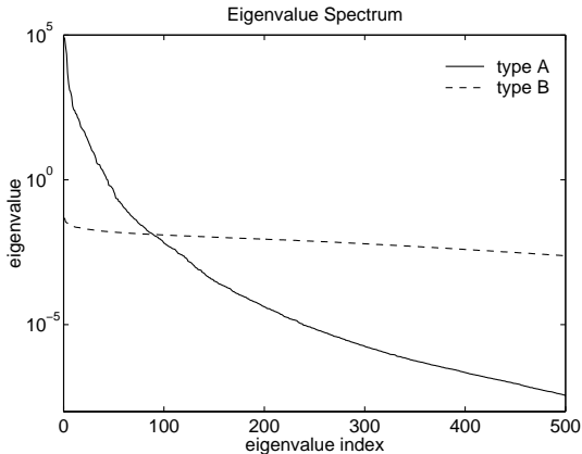
Figure 2. Eigenvalues for the covariance matrices for experiments of type A and B up to eigenvalue index 500. While in type A the spectrum is highly red and 10 modes already explain 99% of the variance in the more realistic setting B 371 modes are required to explain 90% of the variance.
