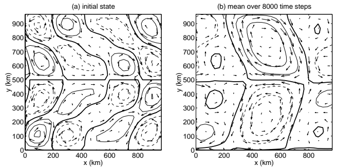
Figure 1. Surface elevation and velocity field (subsamped for displaying) for (a) initial state used for generating the “true” model trajectory and the synthetic observations and (b) mean state over 8000 time steps ( 8 \cdot 10^5 s) using each 10th step. The contour interval is 1 meter. The thick line denotes the mean sea level, dashed lines negative deviations.
