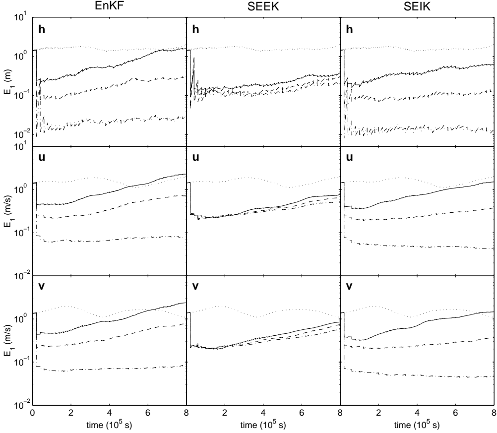
Figure 3. RMS Estimation errors for experiments of type A with poor initial guess. Shown is the time development of the error of the assimilated state for three ensemble sizes ( N=30 (solid line), 100 (dashed), 500 (dash-dotted)) and for a model simulation without assimilation (dotted line). Each column shows the results for one particular filter algorithm. The three rows show the different model fields. For the EnKF and SEIK algorithms divergence can be avoided by large enough ensemble size.
