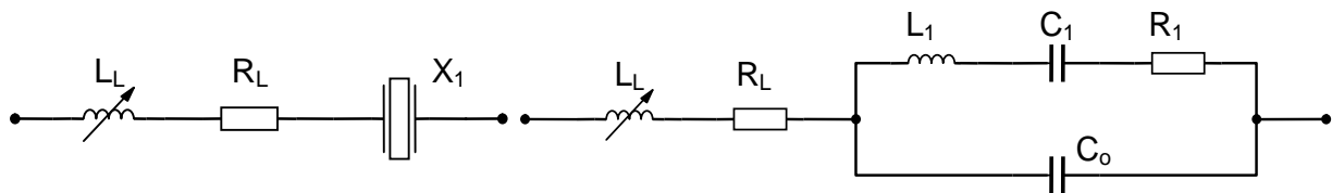
Figure 3. Quartz crystal unit operated with a load inductance.
