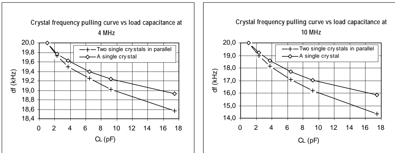
Figure 7. A comparison of pullability exhibited by a single- and dual-crystal unit operated in series with load capacitance at the frequencies of 4 and 10 MHz.
