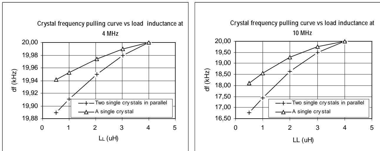
Figure 9. A comparison of pullability exhibited by a single- and dual-crystal unit operated in series with load inductance at the frequencies of 4 and 10 MHz respectively.
