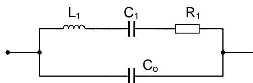
Figure 1. The quartz crystal equivalent circuit.
