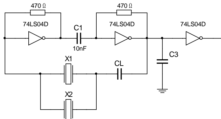
Figure 4. Low-cost TTL oscillator.
