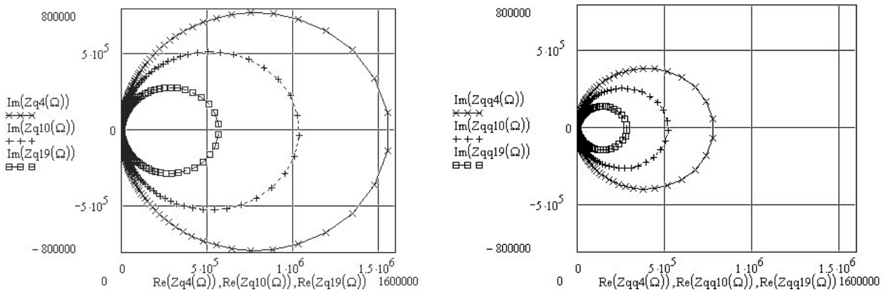
Figure 5. Impedance circles for the oscillation frequencies of 4, 10 and 19 MHz for a single- and dual-crystal unit.
