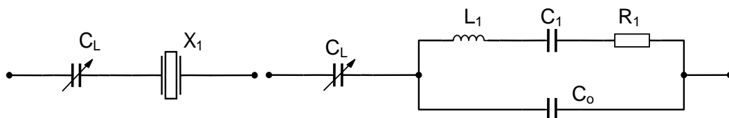
Figure 2. Quartz crystal unit operated with a load capacitance.
