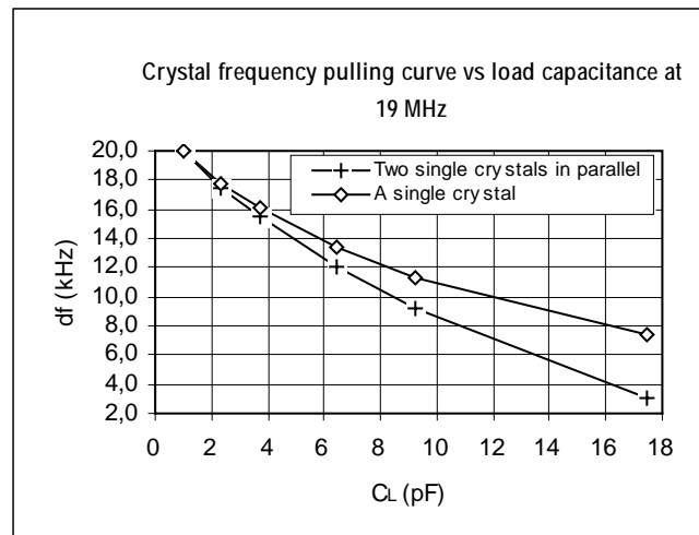
Figure 8. A comparison of pullability exhibited by a single- and dual-crystal unit operated in series with load capacitance at the frequency of 19 MHz.
