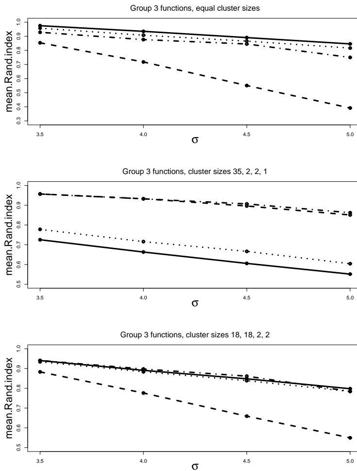
Figure 4: Mean Rand values (averaged over 1000 iterations) for four methods of clustering the Group 3 functions. (Top: Equal cluster sizes. Middle: Cluster sizes 35, 2, 2, 1. Bottom: Cluster sizes 18, 18, 2, 2.) Solid line: Ward's method. Dashed line: Single linkage. Dotted line: Complete linkage. Dot-dashed line: Average linkage.
