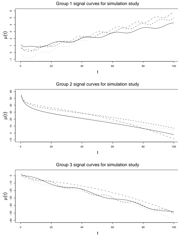
Figure 1: The four signal curves for the three groups of simulated functional data. For each plot: Solid line: \mu_1(t) . Dashed line: \mu_2(t) . Dotted line: \mu_3(t) . Dot-dashed line: \mu_4(t) .
