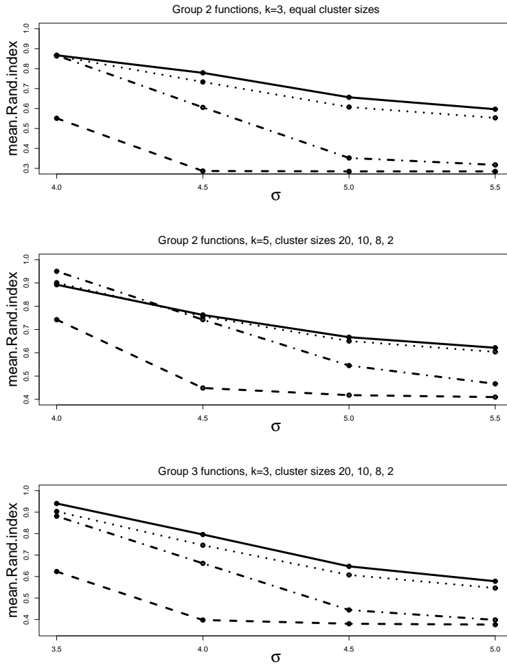
Figure 6: Mean Rand values (averaged over 1000 iterations) for four methods of clustering the Group 2 and 3 functions when misspecifying the number of clusters. (Top: Group 2, Equal cluster sizes, k = 3 . Middle: Group 2, Cluster sizes 20, 10, 8, 2, k = 5 . Bottom: Group 3, Cluster sizes 20, 10, 8, 2, k = 3 .) Solid line: Ward's method. Dashed line: Single linkage. Dotted line: Complete linkage. Dot-dashed line: Average linkage.
