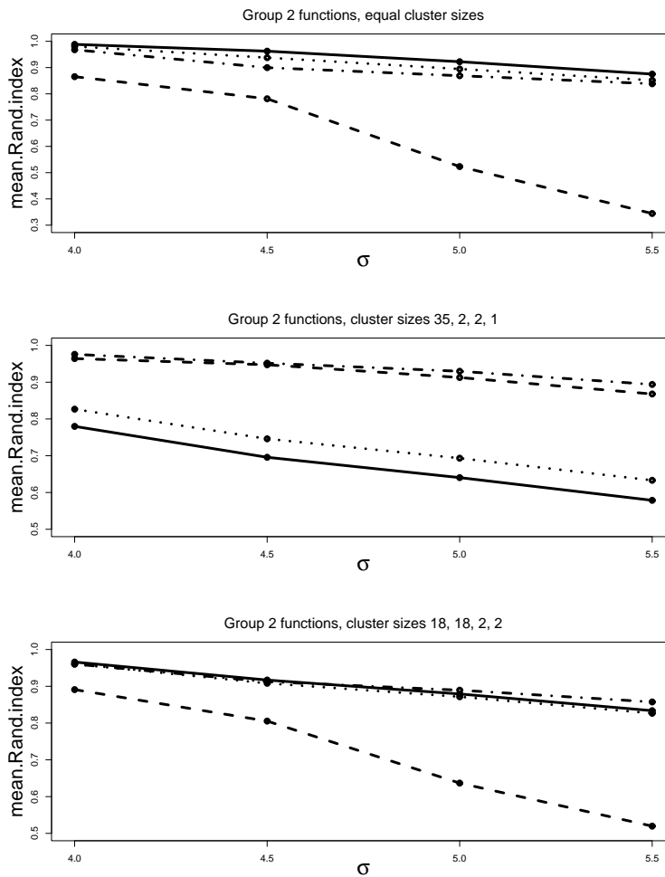
Figure 3: Mean Rand values (averaged over 1000 iterations) for four methods of clustering the Group 2 functions. (Top: Equal cluster sizes. Middle: Cluster sizes 35, 2, 2, 1. Bottom: Cluster sizes 18, 18, 2, 2.) Solid line: Ward's method. Dashed line: Single linkage. Dotted line: Complete linkage. Dot-dashed line: Average linkage.
