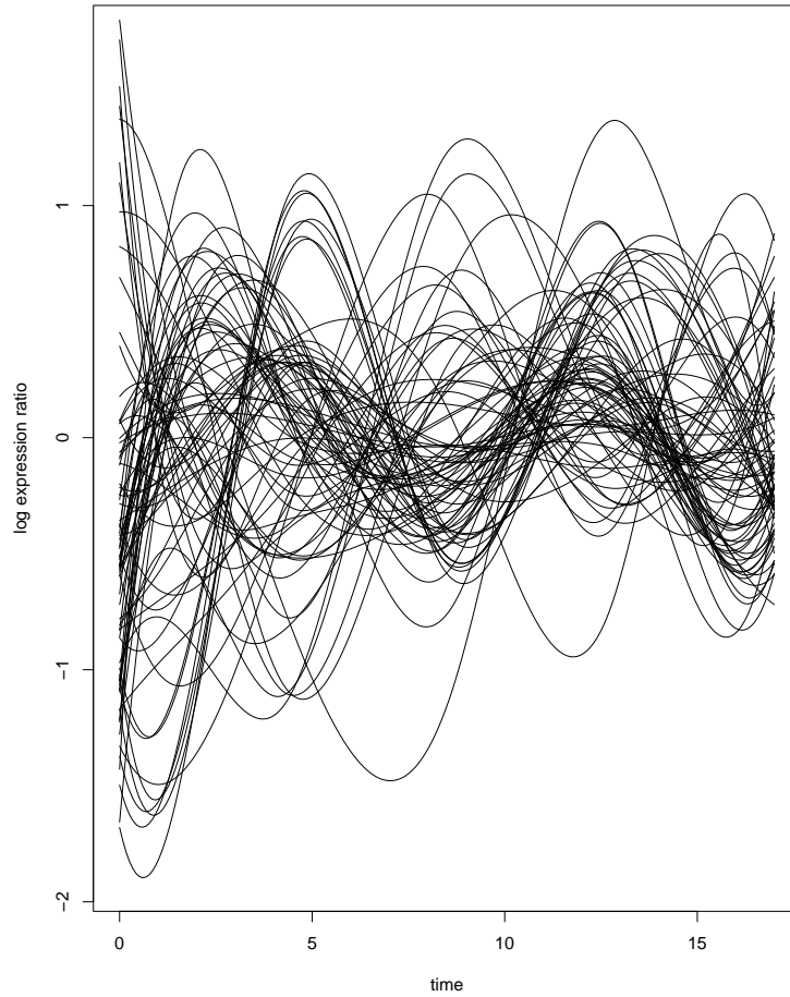
Figure 7: The 78 smoothed and centered curves in the yeast gene data set.
