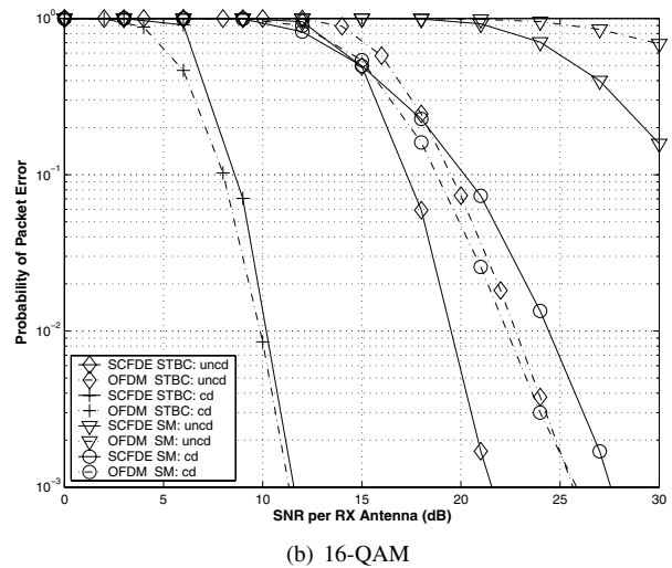
Fig. 2. Packet error rates for STBC and SM systems in the ETSI A channel ( n_t = n_r = 2 ).
