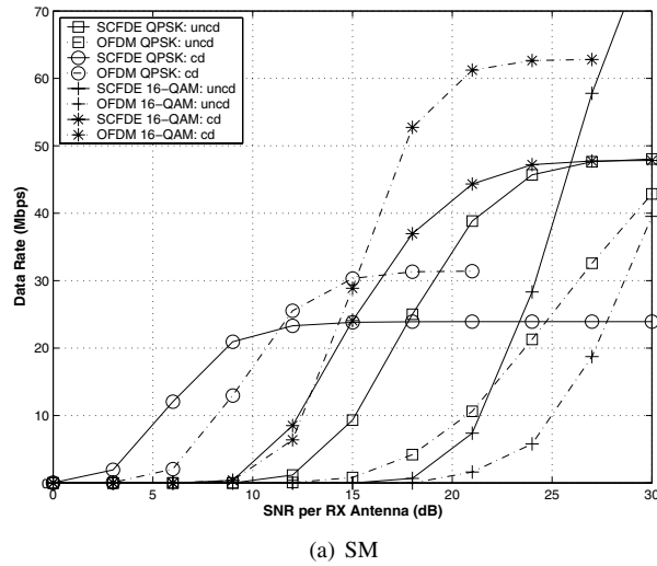
Fig. 4. Throughput for systems in ETSI A channel.
