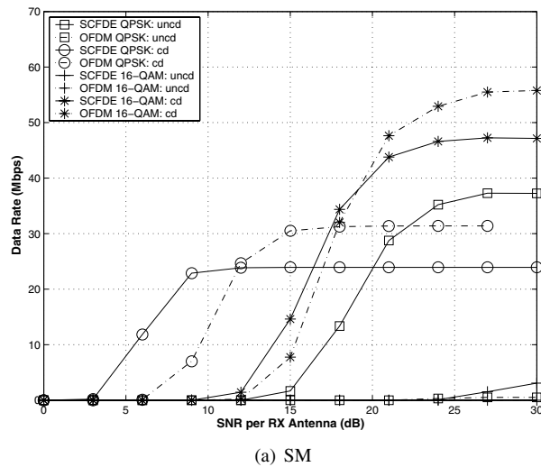
Fig. 5. Throughput for systems in ETSI E channel.
