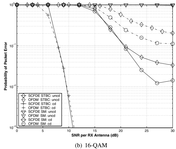
Fig. 3. Packet error rates for STBC and SM systems in the ETSI E channel ( n_t = n_r = 2 ).
