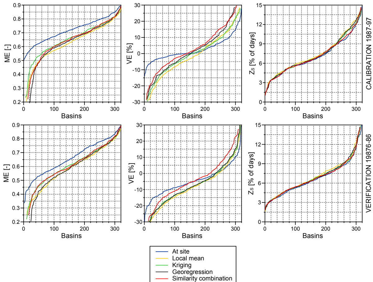
Fig. 8. Summary of the performance of the best regionalisation methods of each group: Cumulative distribution functions ( CDF ) of the model efficiencies of daily runoff ( ME , left), volume errors of runoff ( VE , centre) and percentage of days with poor snow cover simulations ( Z_s , right). 320 basins, calibration (top) and verification (bottom) periods.
