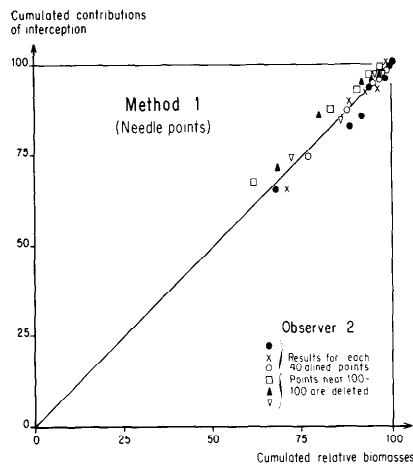
Fig. 4. Relations between relative biomasses and contributions of interception, for species categories, with needle and double metre points.
