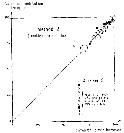
Fig. 4. Relations between relative biomasses and contributions of interception, for species categories, with needle and double metre points.
