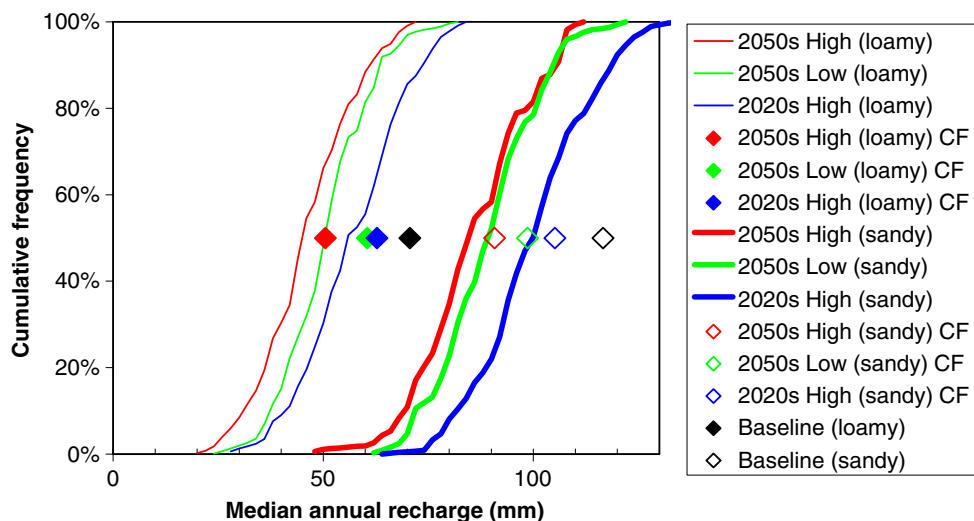
Fig. 4 Cumulative frequency distributions of baseline and future median annual potential recharge at Coltishall for sandy and loamy soils from 100 stochastic and one change factor (CF) simulation for each scenario
