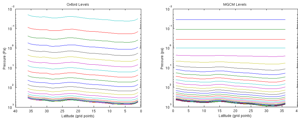
Figure 1: Schematic comparing vertical resolution of the Oxford-LMD Mars model versus the GFDL MGCM. The Oxford model is purely sigma coordinate, whereas the MGCM transitions to pressure coordinates at higher altitudes.
