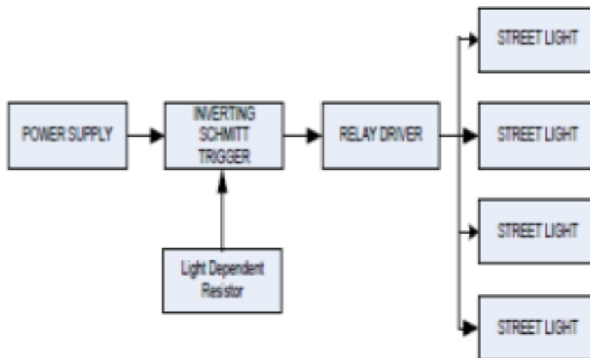
Fig 3 Street Lighting System Using Schmitt Trigger
