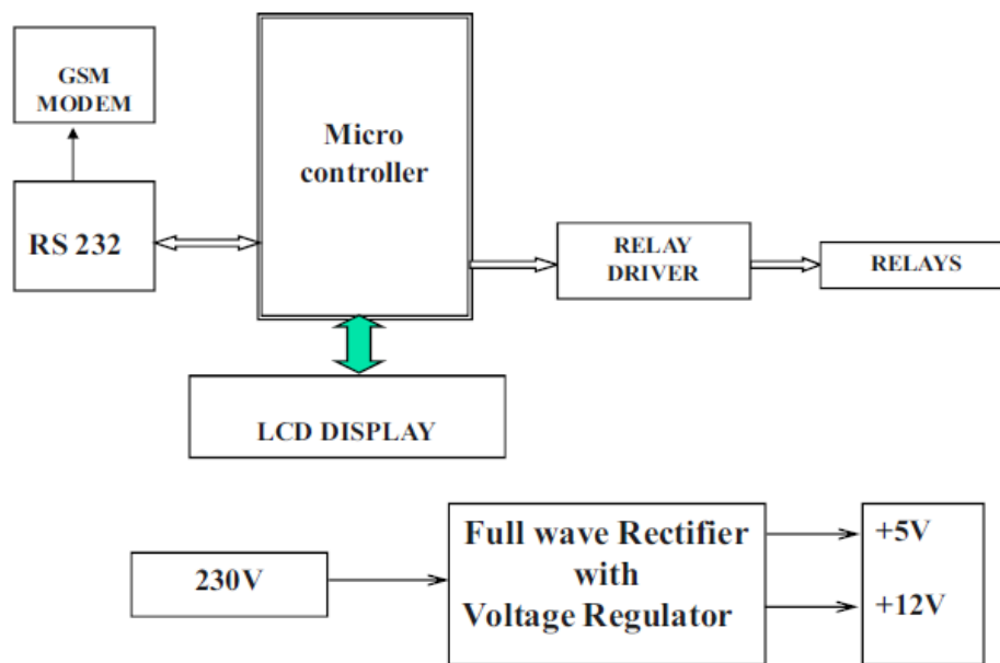
Fig 2 Block Diagram of GSM Based Street Light Automation
