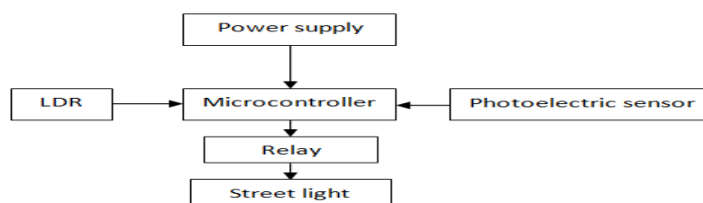
Fig 1. Block diagram of street Light system.
