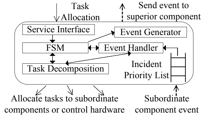
Fig.3 Run-time component model
