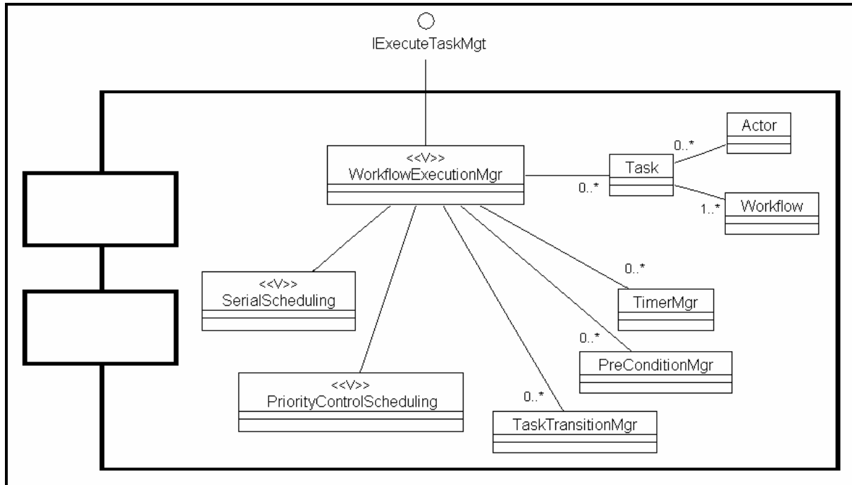
Figure 15: WorkflowExecutionMgr component [32].
