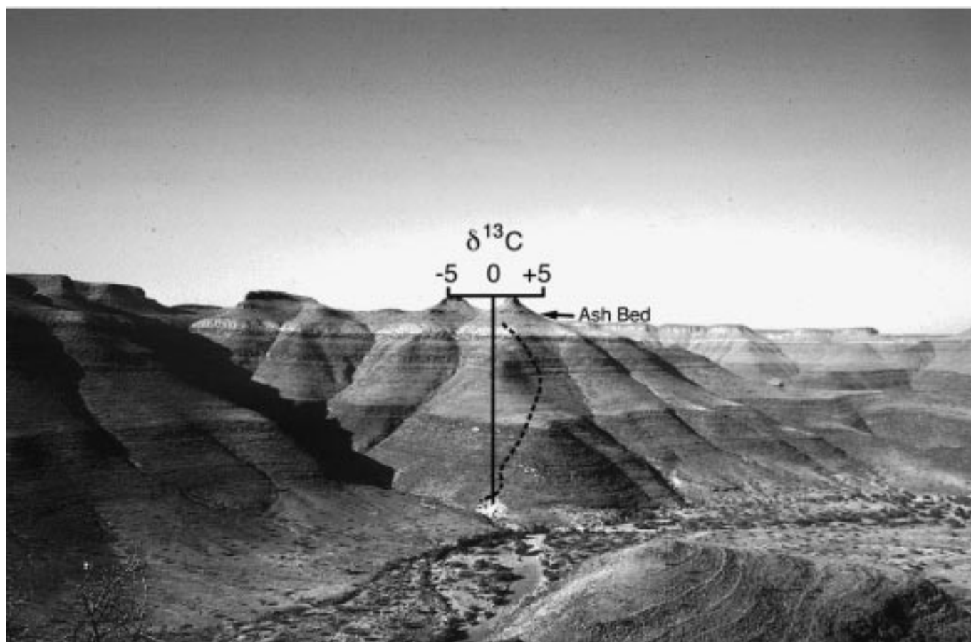
Fig. 5.—Outcrop photograph of the Zebra River section (Fig. 2C) of the Zaris Formation in the northern Nama sub-basin showing position of parasequence boundaries, volcanic ash bed (vvv), and superimposed generalized carbon-isotope profile.
