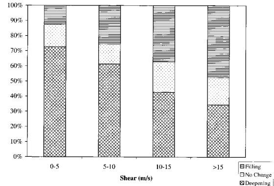
FIG. 2. Percentage of 12-h periods in all storms that are filling, have no change in pressure, or are deepening, as a function of the magnitude of the 850–200-hPa vertical wind shear. This figure incorporates the same tropical cyclones as in Fig. 1, but for 1122 observations times (see section 3a for explanation).
