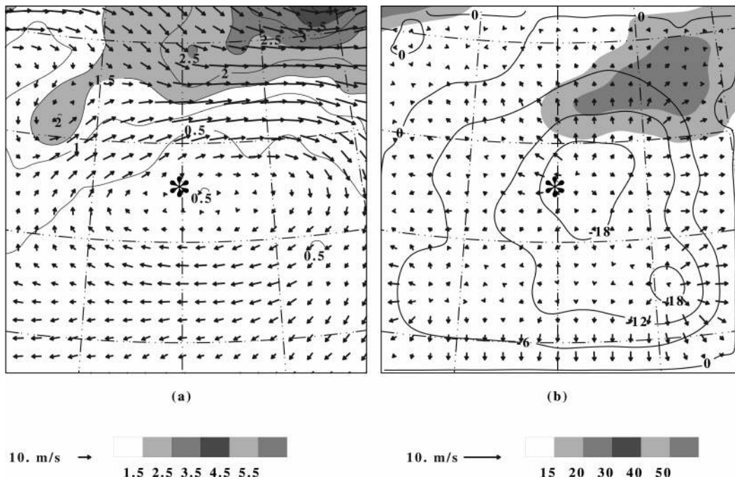
FIG. 8. As in Fig. 7 except for the unfavorable no-trough composite.
