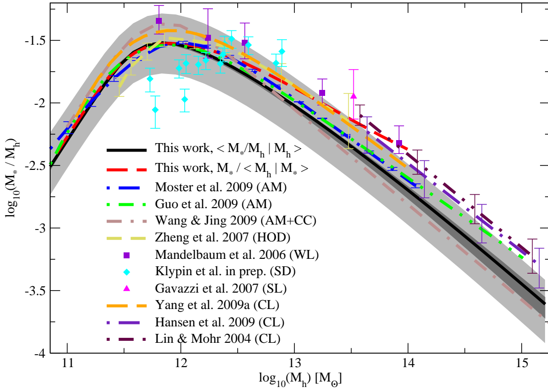
Figure 11. Comparison of our best-fit model at z = 0.1 to previously published results. Results shown include other results from abundance matching (Moster et al. 2009 and Guo et al. 2009); abundance matching plus clustering constraints (Wang & Jing 2009); HOD modeling (Zheng et al. 2007); direct measurements from weak lensing (Mandelbaum et al. 2006), satellite dynamics (Klypin et al. 2009) and strong lensing (Gavazzi et al. 2007); and clusters selected from SDSS spectroscopic data (Yang et al. 2009a), SDSS photometric data (the maxBCG sample Hansen et al. 2009), and X-ray selected clusters (Lin & Mohr 2004). Dark grey shading indicates statistical and sample variance errors; light grey shading includes systematic errors. The red line shows our results averaged over stellar mass instead of halo mass; scatter affects these relations differently at high masses. The results of Mandelbaum et al. (2006) and Klypin et al. (2009) are determined by stacking galaxies in bins of stellar mass, and so are more appropriately compared to this red line.
