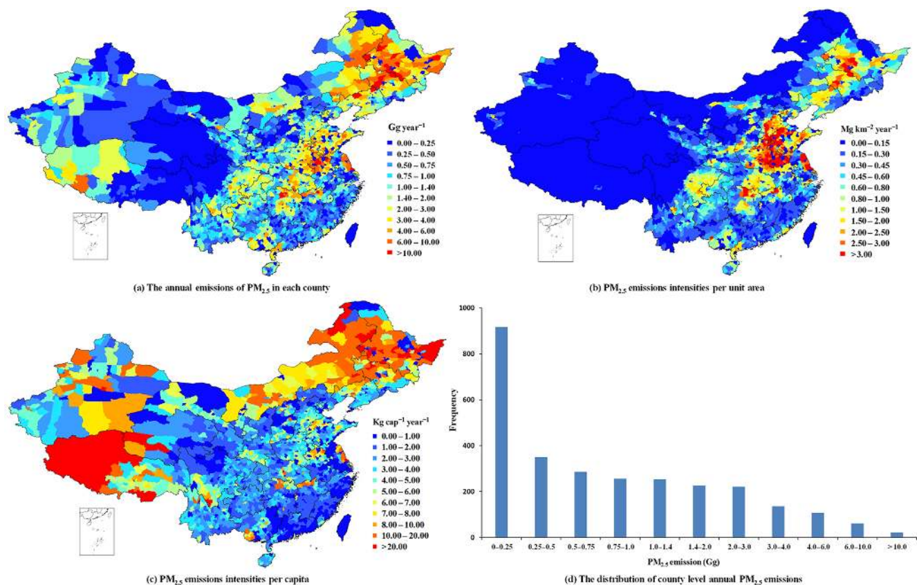
Figure 6. Biomass emission inventory at county resolution and intensity (PM 2.5 ).
