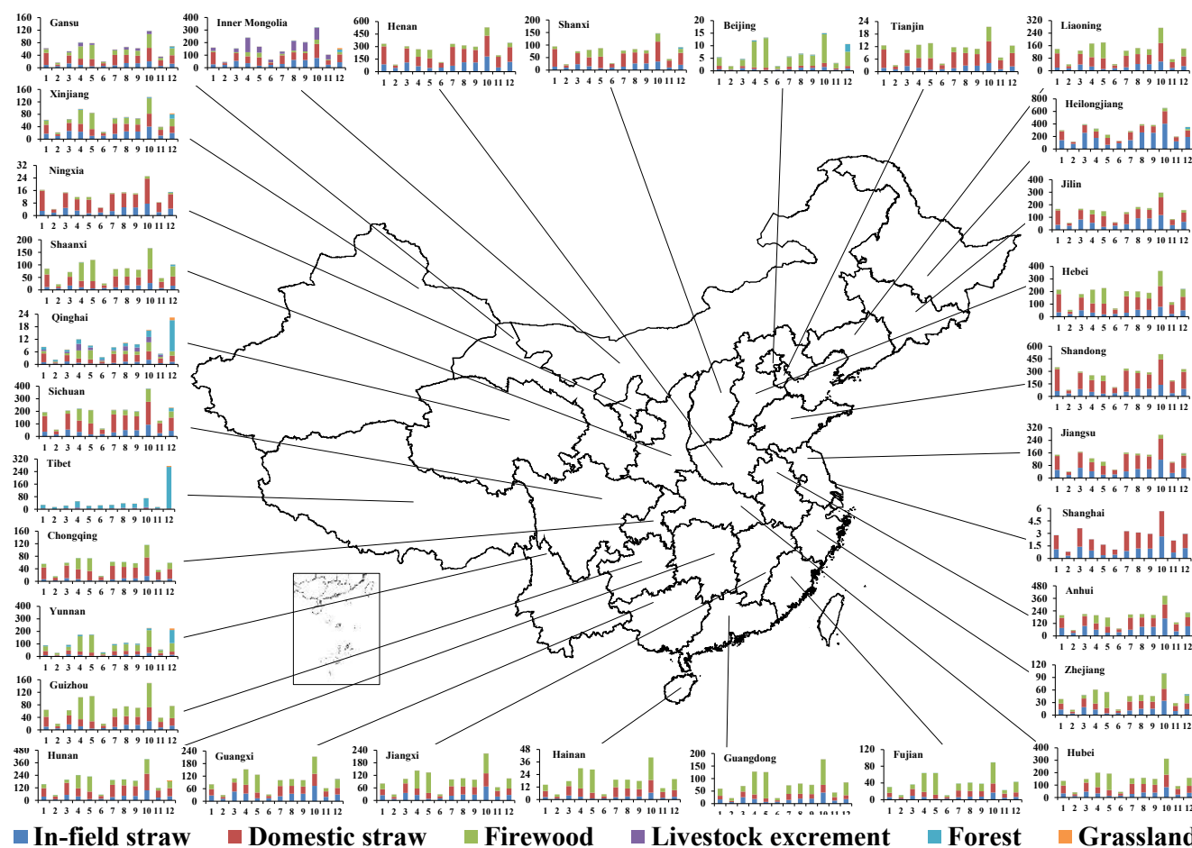
Figure 4. Contributions of different biomass sources to the emission in each province (Gg). Note that numbers 1–12 represent the pollutants of \text{SO}_2 \times 10 , \text{NO}_x , NMVOC, \text{NH}_3 \times 10 , \text{EC} \times 10 , OC, \text{CO}/10 , \text{PM}_{10} , \text{PM}_{2.5} , \text{CO}_2/100 , \text{CH}_4 , and \text{Hg} \times 1\,000\,000 , respectively.
