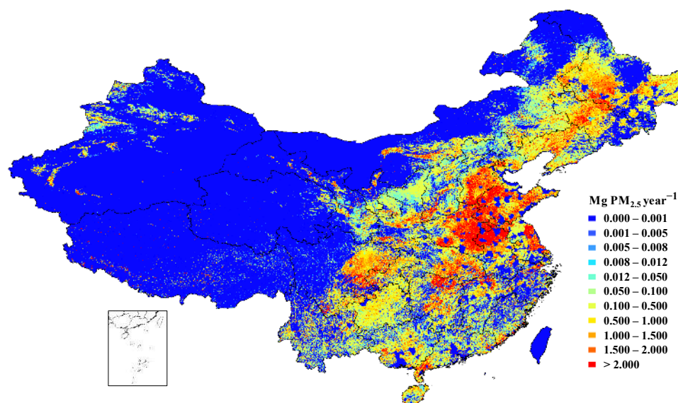
Figure 7. Gridded distribution of PM 2.5 annual emissions.
