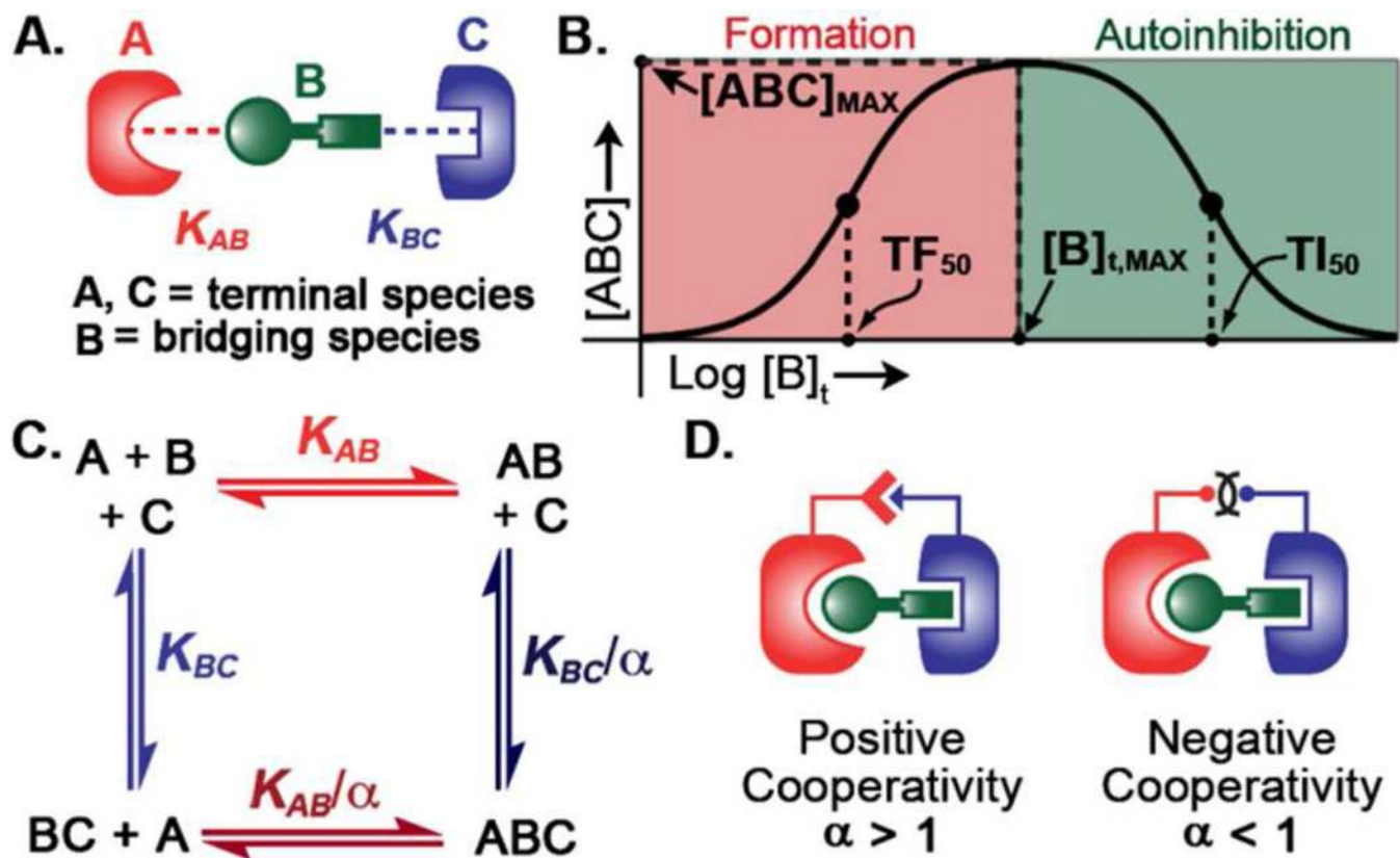
Figure 1. A. Structure of ternary complex and definition of terminology for interacting components. B. Graph depicting ternary complex concentration ( [ABC] ) as a function of total bridging species ( [B]_t ) and illustrating autoinhibition. This curve can be understood in terms of critical points: the maximum concentration of ternary complex that can be achieved ( [ABC]_{max} ), the concentration of [B]_t required to achieve [ABC]_{max} ( [B]_{t,max} ), and the [B]_t values that elicit half-maximal [ABC] formation on the left ( TF_{50} ) and right ( TI_{50} ) sides of the curve. C. Thermodynamic cycle for the reversible formation of ternary complexes. D. Illustrations and mathematical definitions for positive and negative cooperativity.
