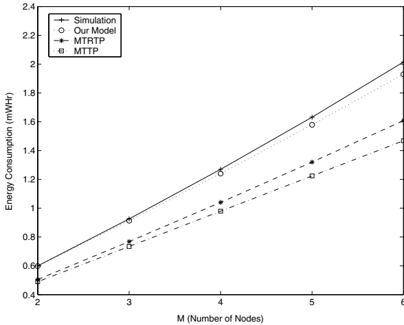
Fig. 5. Energy consumption for simulation and analysis with CSMA.
