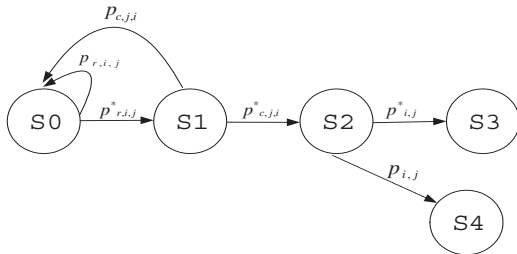
Fig. 2. State diagram for transmitting a packet from node i to node j in MACA.
