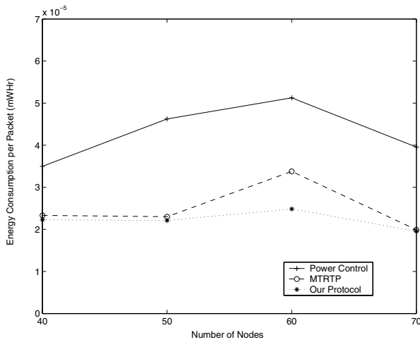
Fig. 11. Energy consumption per packet in two frame scheme.
