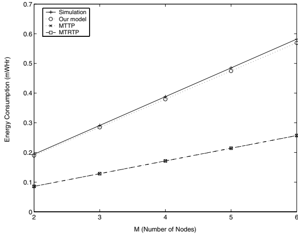
Fig. 8. Energy consumption for simulation and analysis with Four Frame exchange scheme.
