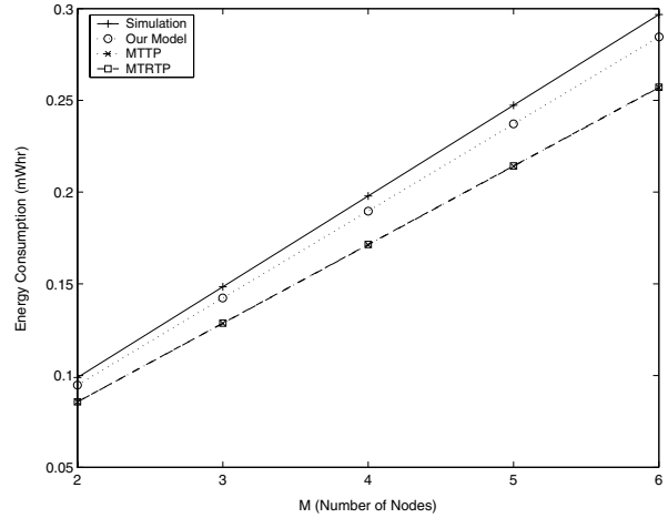
Fig. 7. Energy consumption for simulation and analysis with Two Frame Exchange scheme.
