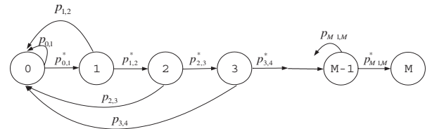
Fig. 1. State diagram for CSMA.
