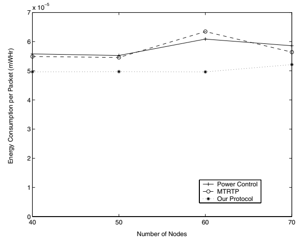
Fig. 9. Energy consumption per packet in MACA.
