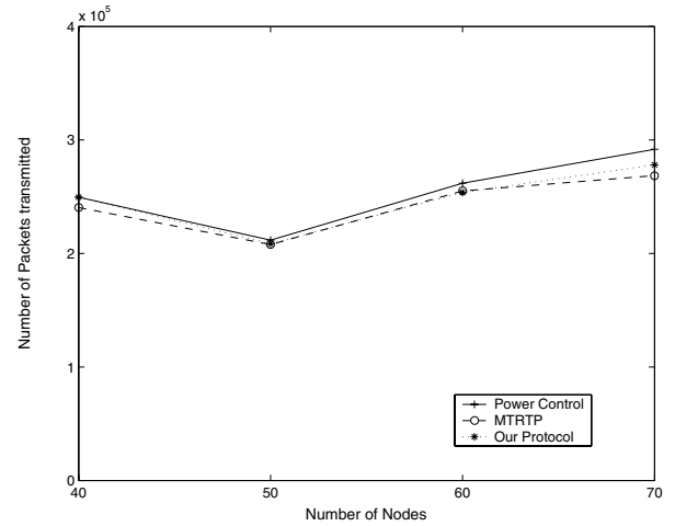
Fig. 10. Number of packets transmitted in MACA.
