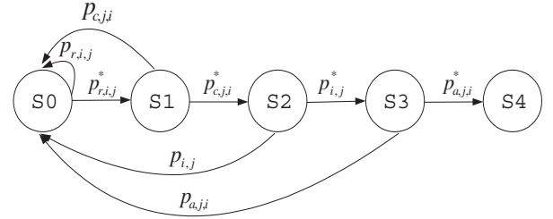
Fig. 4. State diagram for the Four Frame Exchange scheme.
