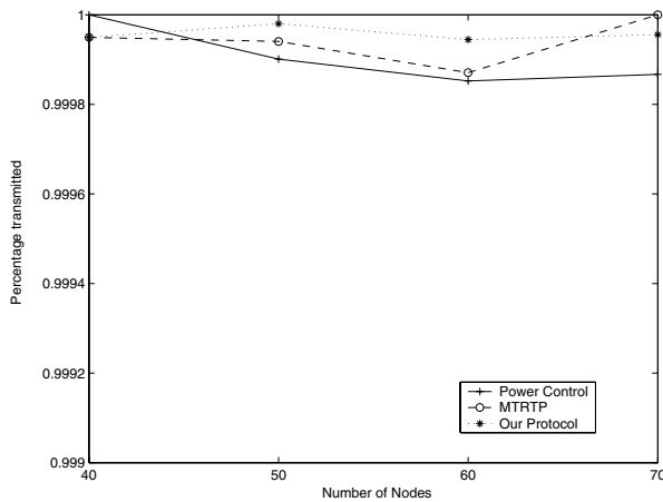
Fig. 12. Percentages of packets transmitted in two frame scheme.
