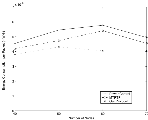
Fig. 13. Energy consumption per packet in four frame scheme.
