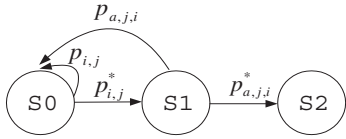
Fig. 3. State diagram for the Two Frame Exchange scheme.
