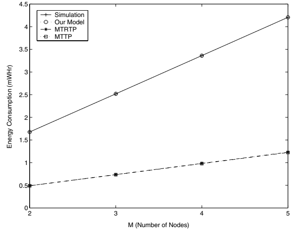
Fig. 6. Energy consumption for simulation and analysis with MACA.
