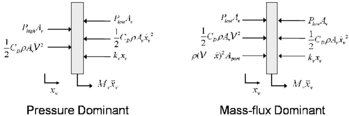
Figure 4: Free body diagrams for the valve reed.
