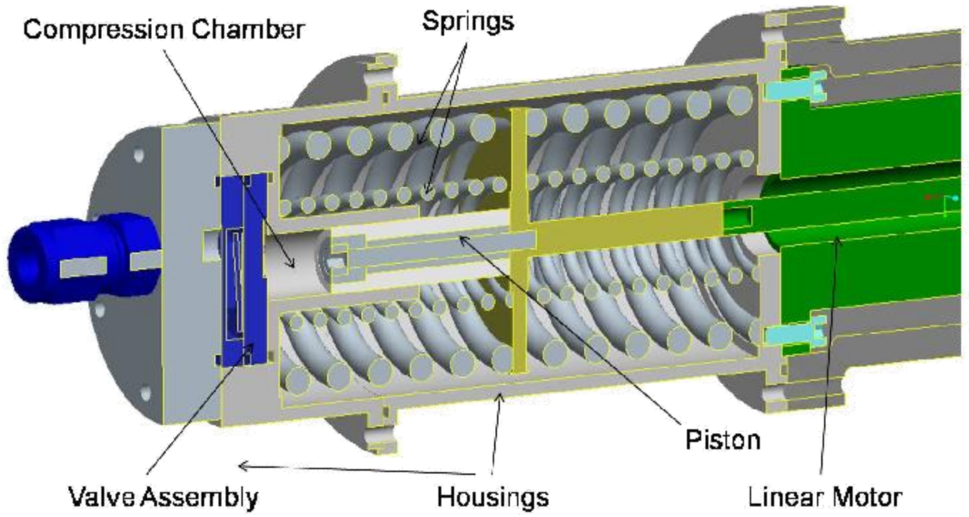
Figure 7: A section view of the prototype linear compressor.
