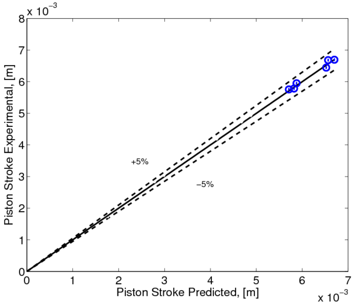
Figure 10: Comparison of experimental and predicted piston displacements.
