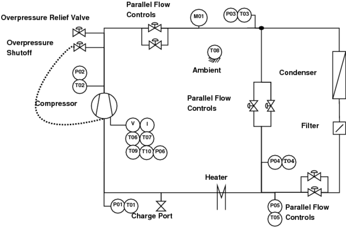
Figure 8: Schematic diagram of miniature-compressor hot gas bypass load stand.
