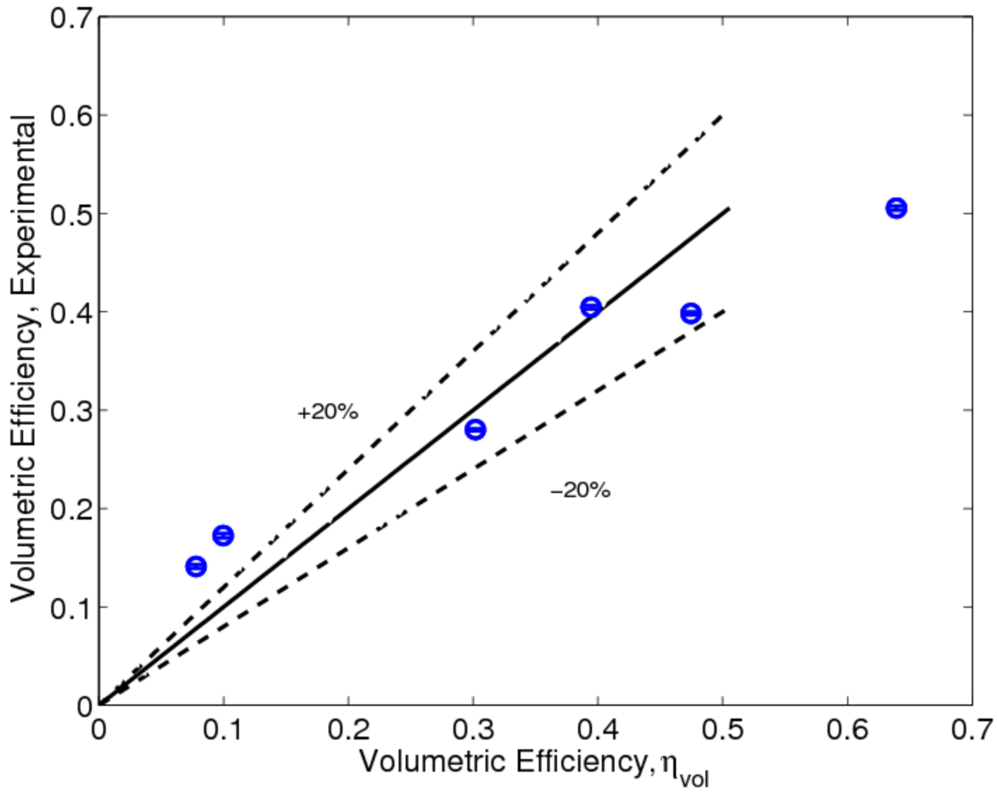
Figure 12: Comparison of experimental and predicted volumetric efficiencies.
