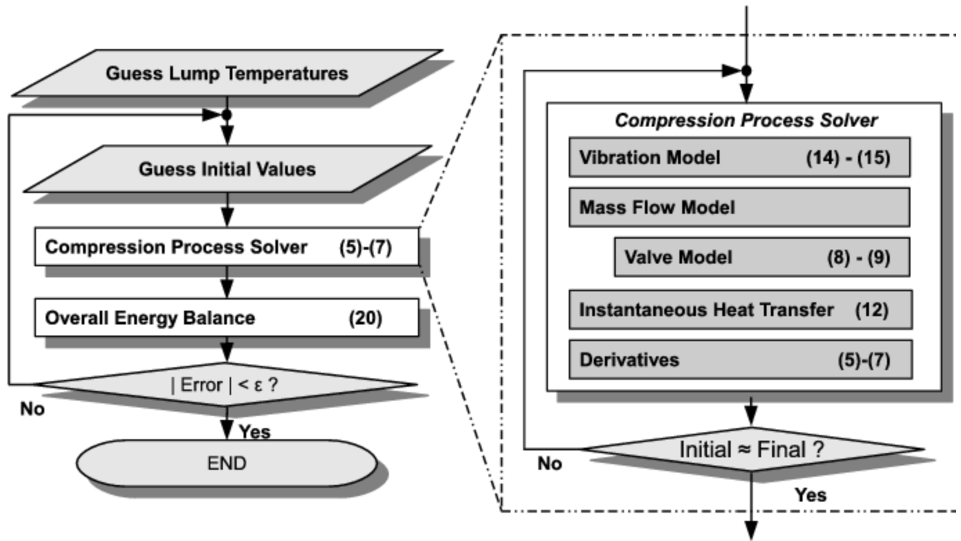
Figure 6: Solution flowchart of linear compressor model (equations solved at each step given in blocks).
