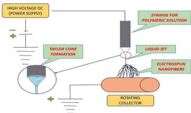
Fig. 6 Diagram shows the formation of Taylor cone in electrospinning technique. 63
