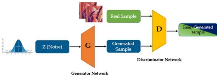
Fig. 14 Graphical representation of the generative adversarial network
