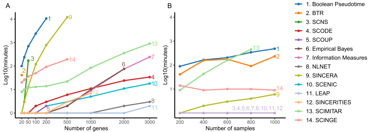
Figure 8. Running time of network inference methods with varying numbers of genes (panel A) and samples (panel B) in the log 10 scale of minutes. Overall, LEAP and NLNET are the fastest methods that can finish every single analysis in minutes.
