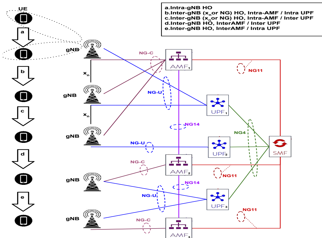
FIGURE 5. 5G mobility architecture based on relevant interfaces and HO use cases. [19]
