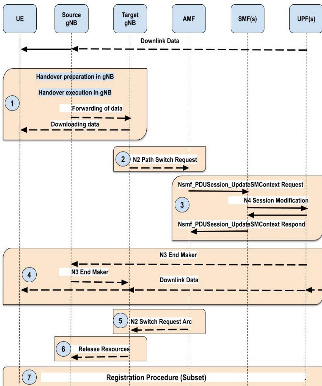
FIGURE 6. X2-based inter-gNB HO [32]
