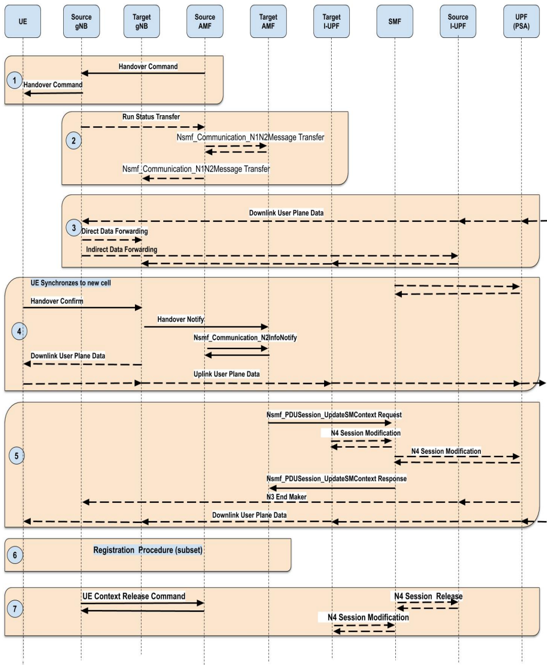
FIGURE 8. Execution phase of N2-based HO [32]
