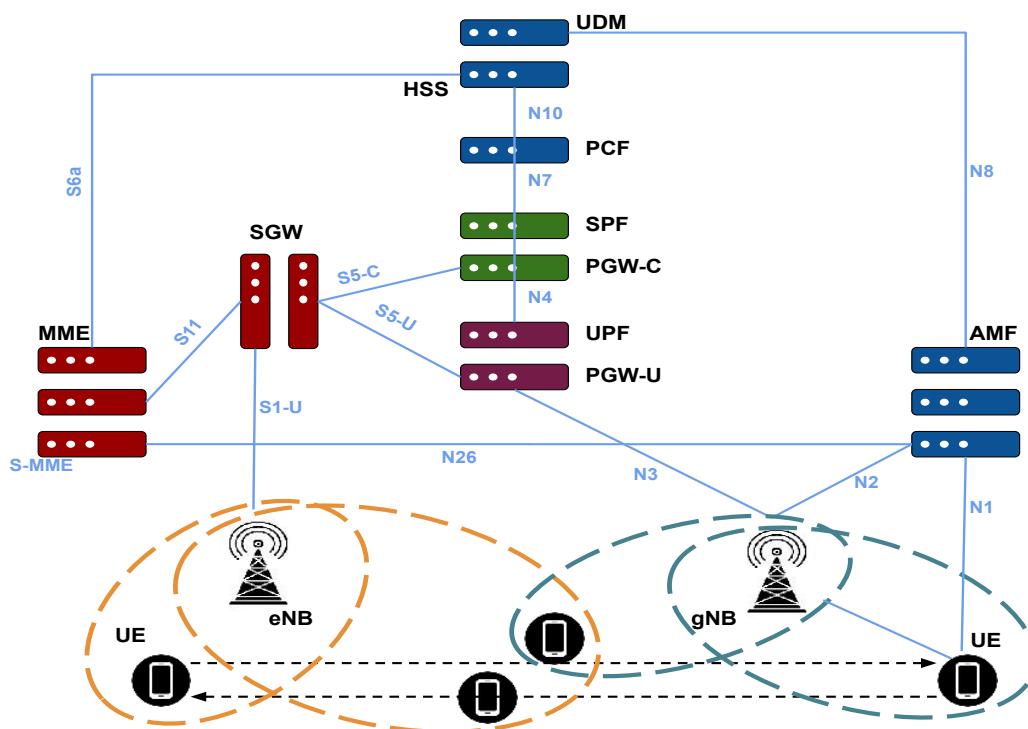
FIGURE 9. HO process from 5G to LTE
