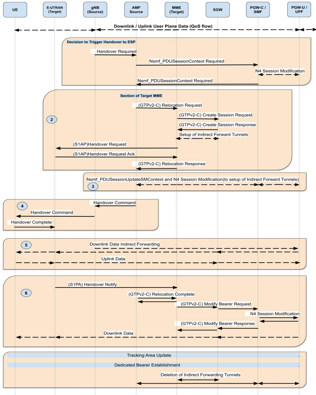
FIGURE 10. Flow chart of HO process from 5G to LTE [32]
