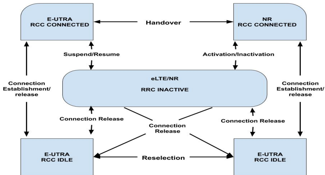
FIGURE 2. RRC state diagram in 5G [24].
