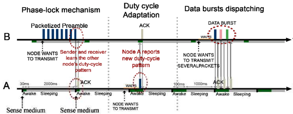
Figure 4. Figure of our proposed MAC layer.
