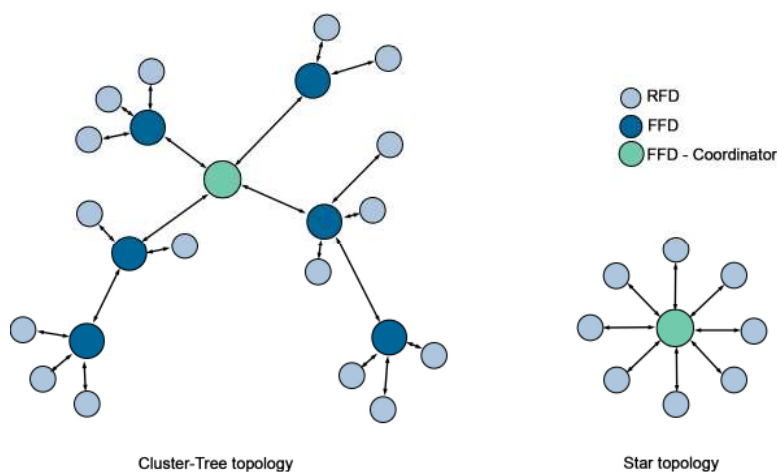
Figure 1. Cluster-Tree and Star topologies.
