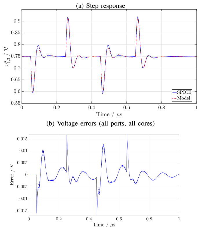
Fig. 16. Transient simulation of the 8-core Server example: (a) step response at a selected port of the first core, and (b) voltage error on all ports of all cores (total 8 \times 57 = 456 error curves).
