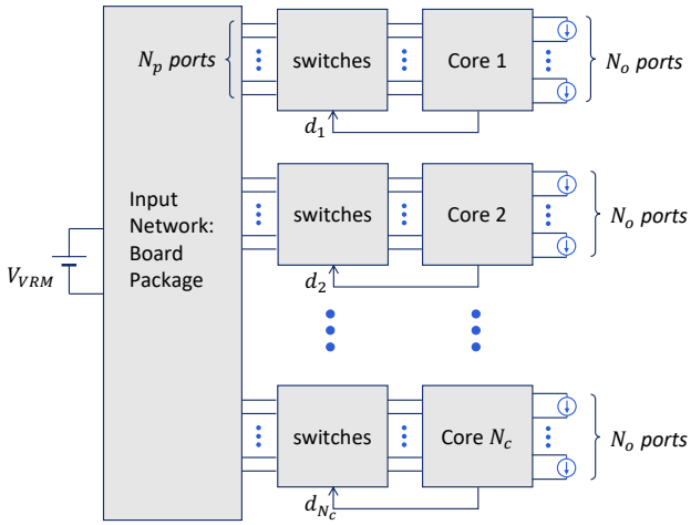
Fig. 1. Schematic illustration of the multicore power distribution system under investigation.
