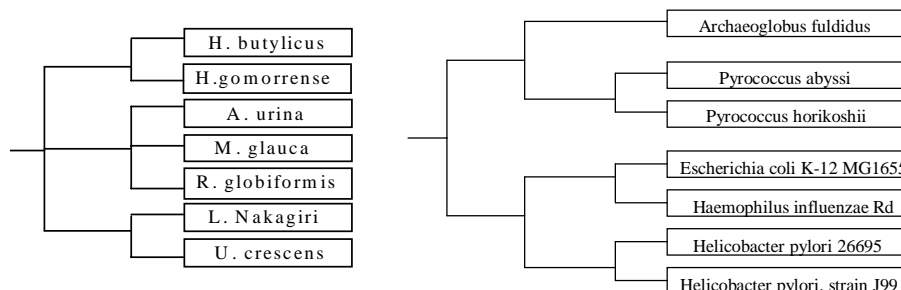
Figure 2: An rRNA tree and a genome tree.
