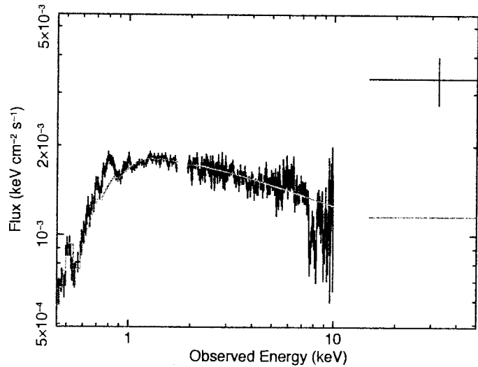
Fig. 6.— The Suzaku XIS and HXD spectra of PDS 456, plotted in \nu F_\nu flux units. A factor of \times 3 excess is seen in the HXD, which may suggest that a Compton thick absorber, with N_{\text{H}} > 10^{24} \text{ cm}^{-2} exists towards this optical type I quasar. The red line shows the extrapolation of the best-fit broken-powerlaw continuum extrapolated to higher energies.
