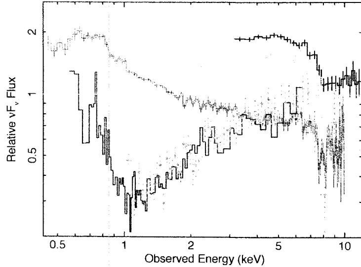
Fig. 8. -- The current observations of PDS 456, shown as \nu F_\nu spectra, where we have plotted the data compared to a ratio with an absorbed ( N_{\text{Gal}} = 2 \times 10^{21} \text{ cm}^{-2} ) power-law of \Gamma = 2 at a mean 2–10 keV flux level of 5 \times 10^{-12} \text{ erg cm}^{-2} \text{ s}^{-1} . Shown are RXTE PCA (black, 1998), XMM-Newton (2001, green), Suzaku XIS (2007, red), Chandra/HETG (2003, blue) and ASCA (1998, orange dotted). Strong variability is seen below 10 keV, from RXTE and XMM at high fluxes, down to Chandra and ASCA as the lowest/hardest observations. Note the 8 keV (observed) Fe K-shell absorption in the XMM 2001, Suzaku 2007 and RXTE 1998 observations. A summary of all these observations is shown in Table 1.
