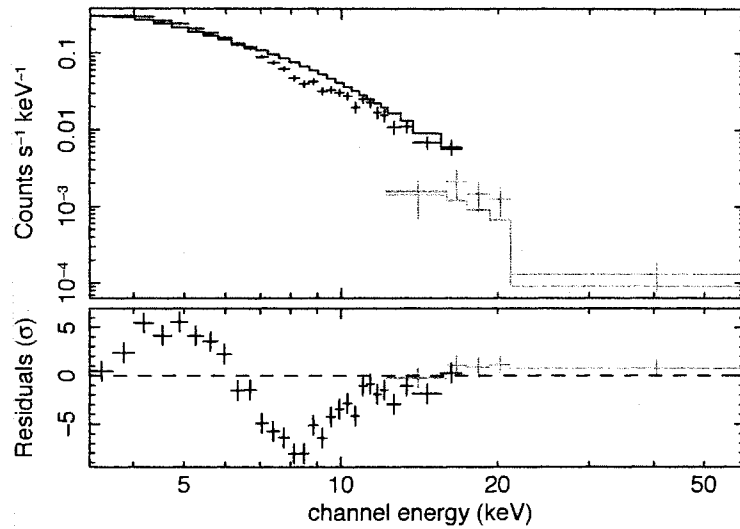
Fig. 10. — A comparison between the time-averaged RXTE/PCA spectrum between 3–18 keV and the HXD/PIN Suzaku spectrum from 15–50 keV. The plot shows the comparison of the data to a \Gamma = 2.2 continuum with Galactic absorption, with no re-normalization of either spectrum, while the lower panel shows the residuals between the data and the model. Although the RXTE/PCA data is non simultaneous with the HXD (see Table 1 for a list of observations), the PCA spectrum below 18 keV extrapolates well to the HXD/PIN data above 15 keV. Also notice the deep absorption trough centered at 8 keV in the RXTE/PCA spectrum, consistent with the absorption in the 2007 Suzaku XIS and 2001 XMM-Newton data.
