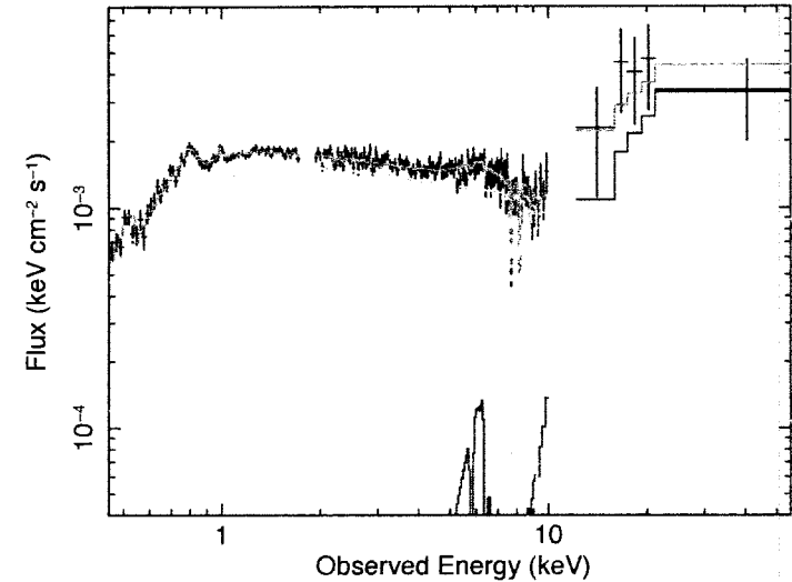
Fig. 9. -- Model fitted to the Suzaku spectrum, representative of absorption and emission from a high column density disk wind, as described in Section 6.3, with model parameters listed in Table 4. Datapoints are shown in black, the dotted green line represents the power-law ( \Gamma = 2.2 ) continuum that is absorbed only by the very high ionization fast outflowing zone, the dark blue line is the continuum obscured by the partial covering absorber which covers 80% of the X-ray source, the light-blue line is the reflected emission off the Compton-thick partially ionized wind and red is the total emission from all components.
