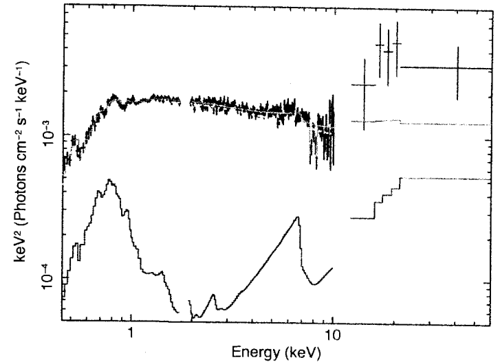
Fig. 7.— Suzaku XIS+HXD spectrum of PDS 456, fitted with an ionized disk reflection model, as described in Section 5.1. Data are shown in black, the blue line shows the blurred reflection component, green shows the intrinsic power-law continuum and red the total emission. Note the HXD/PIN spectrum is more finely binned than in Figure 6, at \sim 2\sigma per bin above the background level.
