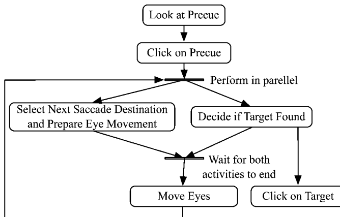
FIGURE 6. Flowchart of the production rules for the process-monitoring strategy.
