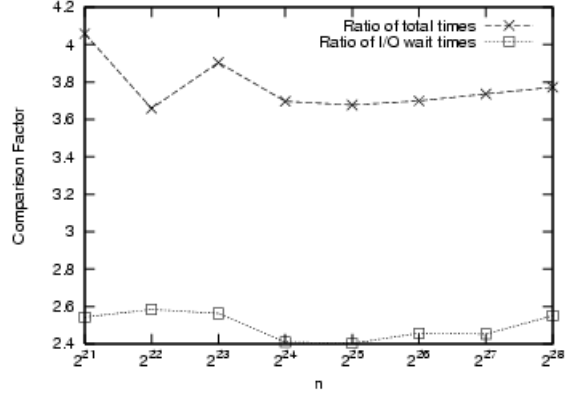
Figure 5: Variation of comparison factor (MM_BFS/MR_BFS) of running time and I/O wait time with random-graph size
