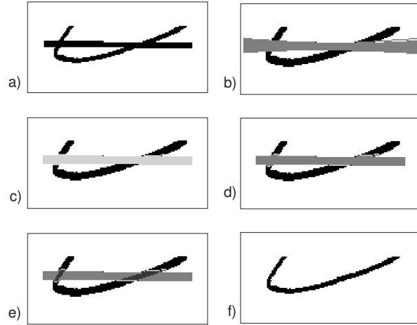
Fig. 16. Proposed line reconstruction: (a) binarized image, (b) searching for line candidates, (c) detected line, (d) line removal with concomitant stroke marking, (e) reconstructed line, (f) result image
