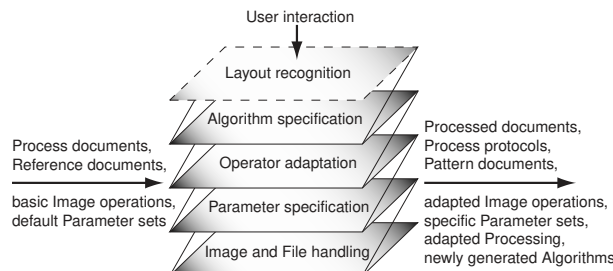
Fig. 7. Layer model of the framework for document processing
