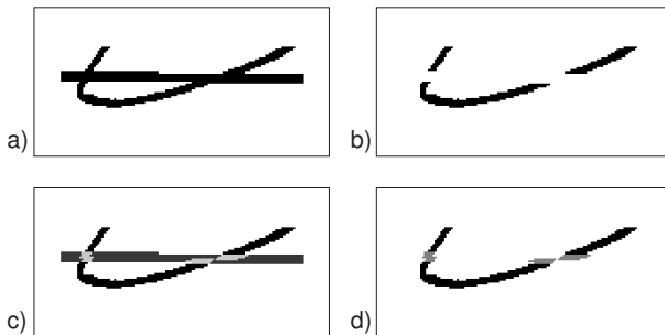
Fig. 15. Line reconstruction by using morphological filtering (length of the structuring element = 5 pixels; angle = \pi/4 ): (a) binarized image, (b) stroke image after line removal, (c) reconstructed stroke, (d) result image
