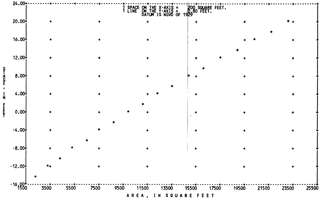
Figure 4.--Sample program-generated line-printer plot of stage-dependent cross-sectional area.
