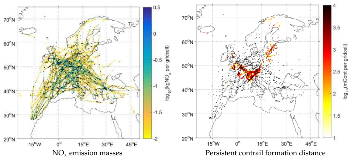
Figure 5. NO x emissions (left) and persistent contrail formation distance (right) per gridcell (0.25° × 0.25°) integrated over a time period of 20 s on 18 December 2015, 12:00 p.m. UTC. Single aircraft are represented as black dots (1216 in total). Note that a low pass filter was applied to the distributions in order to visualise the prior flight path.
