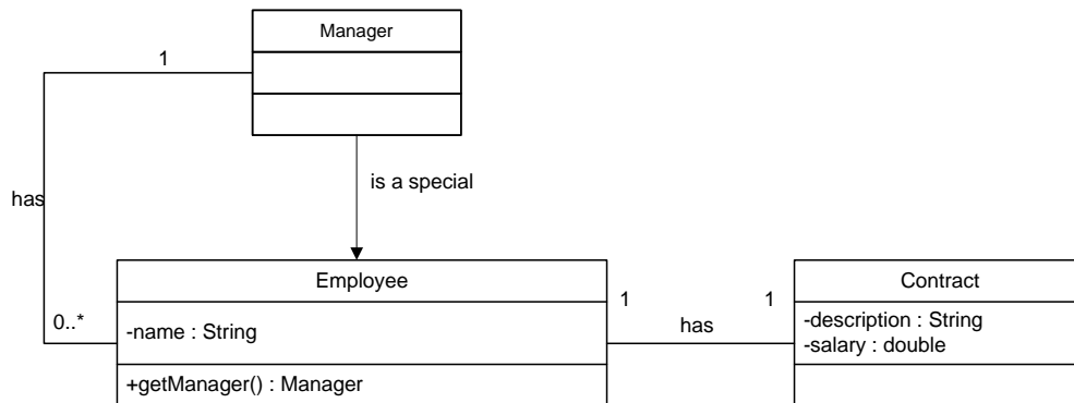
Figure 1: Types of relations in OO
