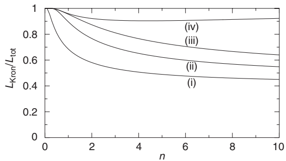
Figure 10 Kron luminosity within 2.5R_1 , normalised against the total luminosity, as a function of the underlying light-profile shape n . The different curves arise from the different values of R_1 obtained by integrating Equation (31) to (i) 1R_e , (ii) 2R_e , (iii) 4R_e , and (iv) infinity.
