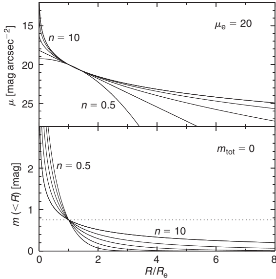
Figure 1 Top panel: Sérsic surface brightness profiles (Equation 6) for n = 0.5, 1, 2, 4, and 10 . The profiles have been normalised at \mu_e = 20 \text{ mag arcsec}^{-2} . Bottom panel: Sérsic aperture magnitude profiles (Equation 5), normalised such that the total magnitude equals zero. The dotted line is offset by 0.75 \text{ mag} (a factor of 2 in flux) from the total magnitude.
