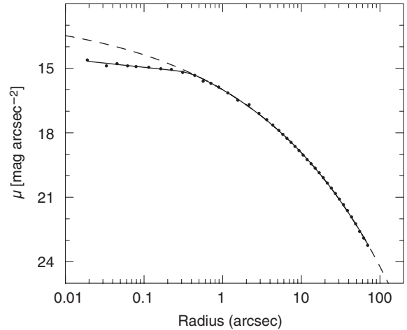
Figure 11 Major-axis, R -band light-profile of NGC 3348. The solid line is the best-fitting core–Sérsic model while the dashed line is the best-fitting Sérsic model to the data beyond the HST -resolved break radius (Graham et al. 2003a,b; Trujillo et al. 2004).
