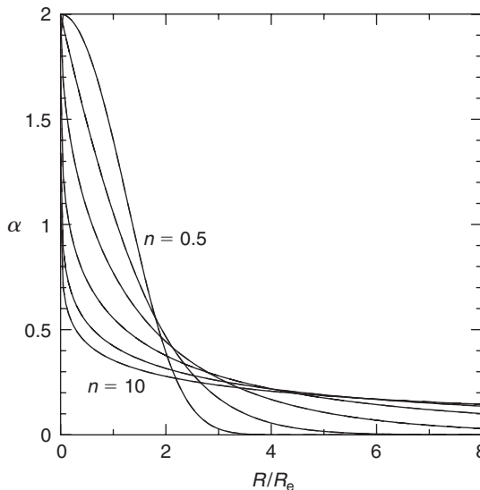
Figure 5 The slope \alpha (Equation 25) is shown as a function of normalised radius R/R_e for n = 0.5, 1, 2, 4, and 10 .
