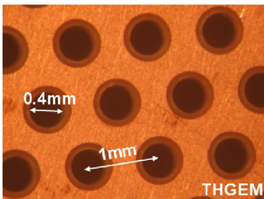
Fig. 1. Photograph of a typical THGEM electrode; the one shown has a hole-diameter of d = 0.4 mm with 0.1 mm etched rim, spaced by a = 1 mm. The thickness is t = 0.5 mm.
