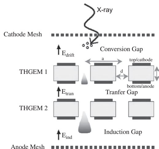
Fig. 3. Schematic view of a double-THGEM soft X-ray detector; the same configuration is adequate for particle tracking and timing.
