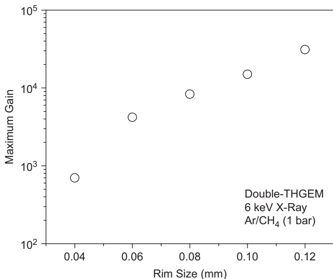
Fig. 2. Maximum attainable gain vs. rim size. Detector parameters: t = 0.4 mm; a = 1 mm; d = 0.3 mm.
