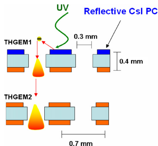
Fig. 5. Schematic view of a double-THGEM with a reflective CsI photocathode deposited on the top one. Photoelectrons are efficiently focused into THGEM1 and multiplied in two steps.
