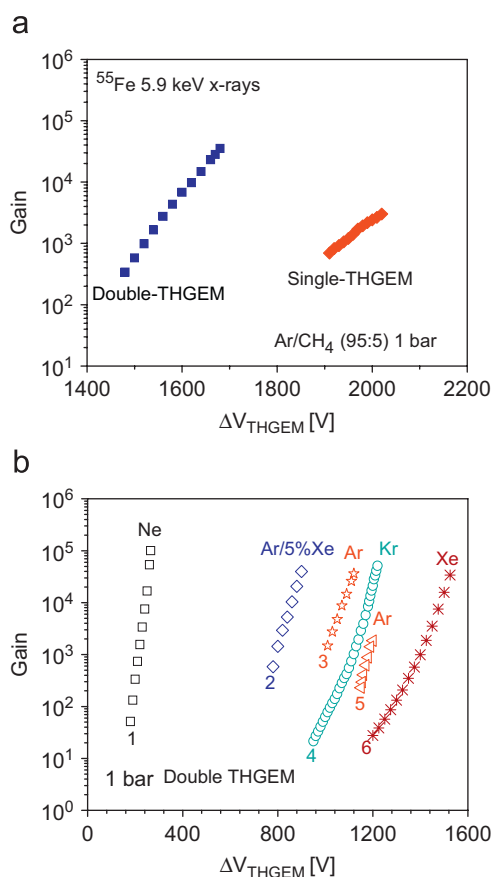
Fig. 4. Gain curves with 5.9 keV X-rays. (a) In single- and double-THGEM ( t = 0.8 mm, d = 0.6 mm, a = 1 mm) in 1 bar Ar/5%CH 4 and (b) in double-THGEM in noble gases at 1 bar. In (a), except for Ar curve (3), measured in gas-flow mode (not purified), all other data were measured with getter-purified gases [18].
