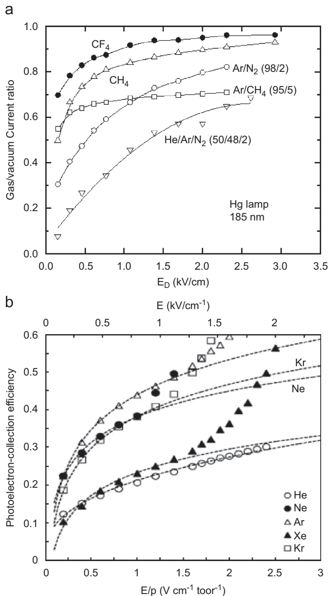
Fig. 10. Measured photoelectron collection efficiency into different gases vs. electric field in: (a) molecular gases and gas mixtures [26] and (b) noble gases. In the latter the dashed lines are model-calculated; the divergence measured in Ar, Kr, Ne and Xe for E > 1.2 kV/cm originates from gas excitation onset [27].
