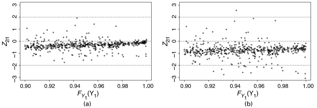
Fig. 4. Diagnostic plots for data from the bivariate extreme value distribution with asymmetric logistic dependence structure—scatterplots of residuals Z_{2|1} against the conditioning variable Y_1 , after transforming Y_1 to uniform margins: (a) residuals from fitting the weakly pairwise exchangeable model; (b) residuals from fitting the asymmetric conditional model
