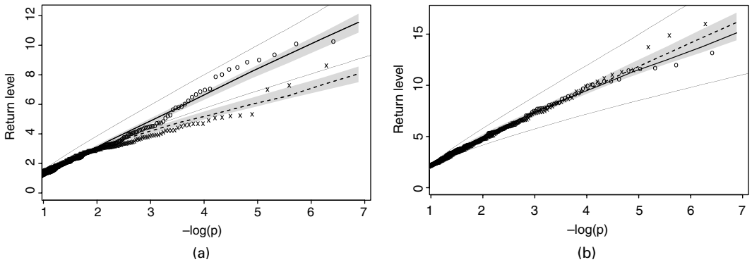
Fig. 7. Return level estimates for the set C^m(v) , for \mathcal{M} corresponding to (a) ( O_3, NO_2 ) and (b) ( NO_2, SO_2, PM_{10} ): —, point estimates for summer; - - - - -, point estimates for winter variables; ■, pointwise 95% confidence intervals (which overlap in (b)); ○, empirical points for summer; ×, empirical points for winter; —, return levels calculated under perfect dependence (upper) and exact independence (lower)
