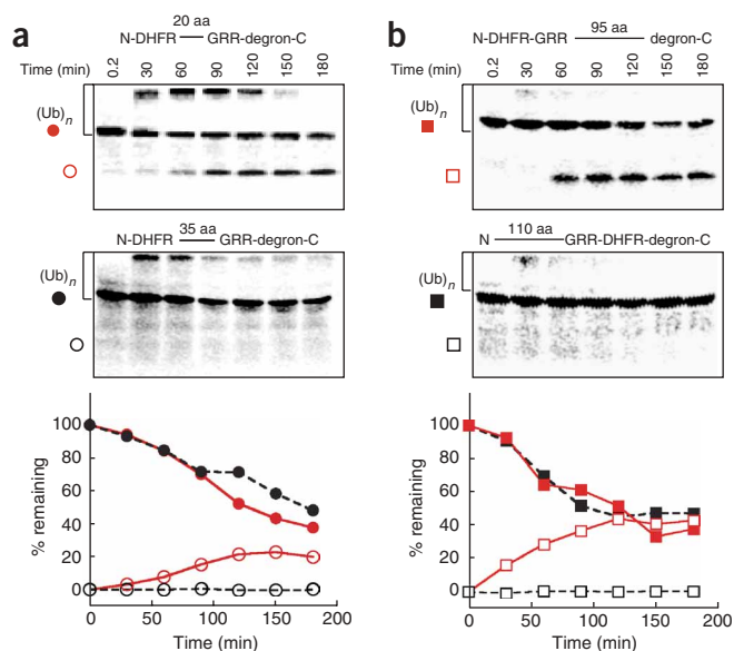
Figure 3 The spacing of the simple sequence inserts relative to the folded domain determines fragment formation. ^{35}\text{S} -labeled fusion proteins were degraded by the proteasome from a C degron at 30 °C. The extent of degradation and fragment formation was quantified as in Figure 1 .
