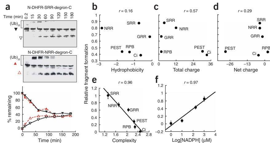
Figure 2 Progression of proteasomal degradation can be inhibited by simple sequences. (a) Fusion proteins containing an SRR (solid black triangle) or an NRR (solid red triangle) were degraded by the proteasome, which led to the accumulation of fragments (SRR, open black triangle; NRR, open red triangle). The extent of degradation and fragment formation was quantified and plotted as in Figure 1. (b–f) The amount of fragment formation is correlated with both the complexity of the simple sequence insert and the stability of the folded domain. Relative fragment formation represents the amount of fragment formed in the presence of 10 \mu\text{M} NADPH relative to the amount of full-length protein degraded. Relative fragment formation for substrates with six different simple sequence inserts was plotted according to the hydrophobicity (b), total charge (c), net charge (d) and amino acid–sequence complexity (e) of the simple sequence and according to the stability of the folded domain (f). The simple sequences used were SRR, NRR, GRR, the repeat region from the C terminus of RNA polymerase II (RPB), the PEST domain from I \kappa B \alpha (PEST) and the Ci cleavage region (Ci).
