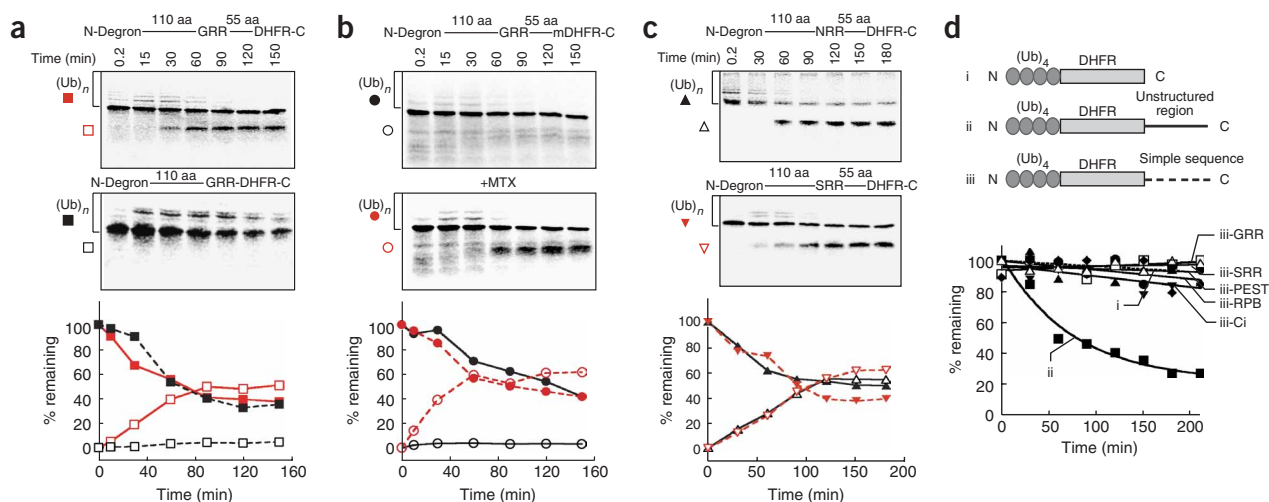
Figure 4 Simple sequence inserts can inhibit proteasome progression in both directions of degradation. Simple sequences do not function as efficient degradation initiation sites. ^{35}\text{S} -labeled fusion proteins were degraded by the proteasome from an N-terminal degron (N degron) at 30 °C. The extent of degradation and fragment formation was quantified as in Figure 1 . (a) Substrate protein containing an N degron followed by a glycine-rich insert, a 55-residue spacer and an E. coli DHFR domain (solid red square) was degraded by the proteasome, which resulted in the accumulation of partially degraded product (open red square) corresponding in size to the DHFR domain plus ~80 residues as judged by its gel mobility (not shown). Placing the GRR insert adjacent to the N terminus of DHFR by removing the spacer region abolished fragment formation (full-length protein, solid black square). (b) When E. coli DHFR was replaced with the less stable mouse homolog (mDHFR, solid black circle), the proteasome degraded the substrate protein completely and no fragment accumulated (open black circle). Stabilizing mDHFR with 320 \mu\text{M} MTX restored fragment formation (full-length protein, solid red circle; fragment, open red circle). (c) The GRR insert can be replaced with an asparagine-rich (solid black triangle) or serine-rich (solid red triangle) sequence without reducing the accumulation of partially degraded product (NRR, open black triangle; SRR, open red triangle). (d) Degradation of a fusion protein consisting of four ubiquitin sequences fused in frame to E. coli DHFR by the proteasome at 25 °C. Construct i lacked an extended unstructured region that could serve as a degradation initiation site and was therefore hydrolyzed only inefficiently. Degradation was accelerated when an unstructured region was attached to the C terminus of the protein (ii). However, proteins with hydrophilic simple sequences (GRR, SRR, PEST, RPB or Ci, defined as in Figure 2 ) fused to their C termini as initiation sites (iii) were not degraded.
