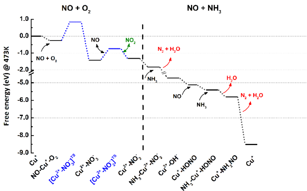
Figure 3: Calculated free energy diagram for the NO activation cycle shown in Scheme 1. The free energies at each level are given relative to Z\text{-Cu}^+ , and the appropriate gas phase molecules. Calculated activation energies in the oxidation part are shown in blue.
